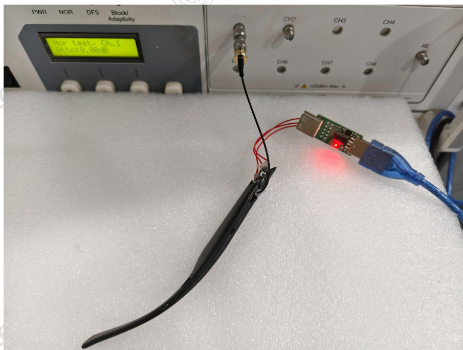
Band edge emissions (Radiated) Radiated emissions (above 1GHz)
