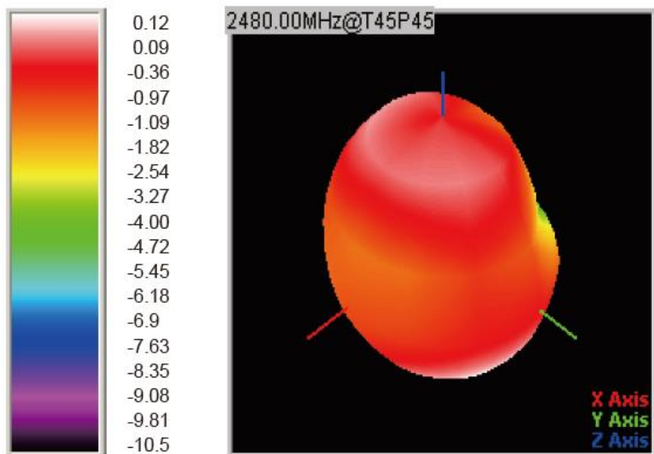
© 3D Gain Pattern (2480 MHz)
