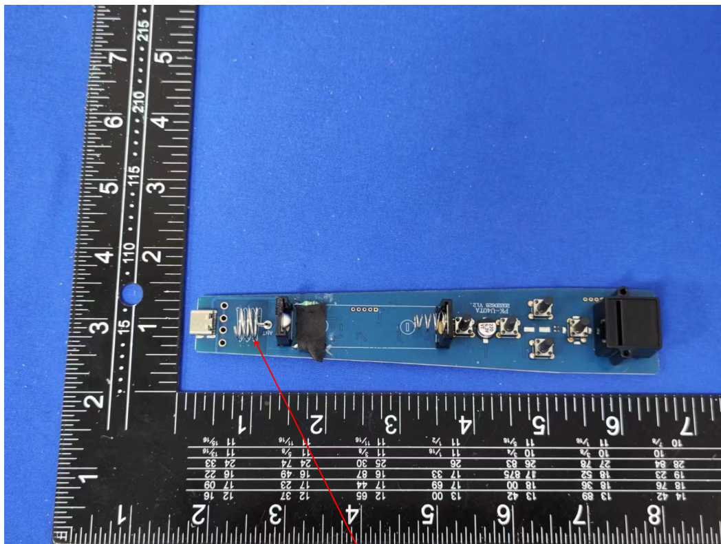
Spring Antenna
