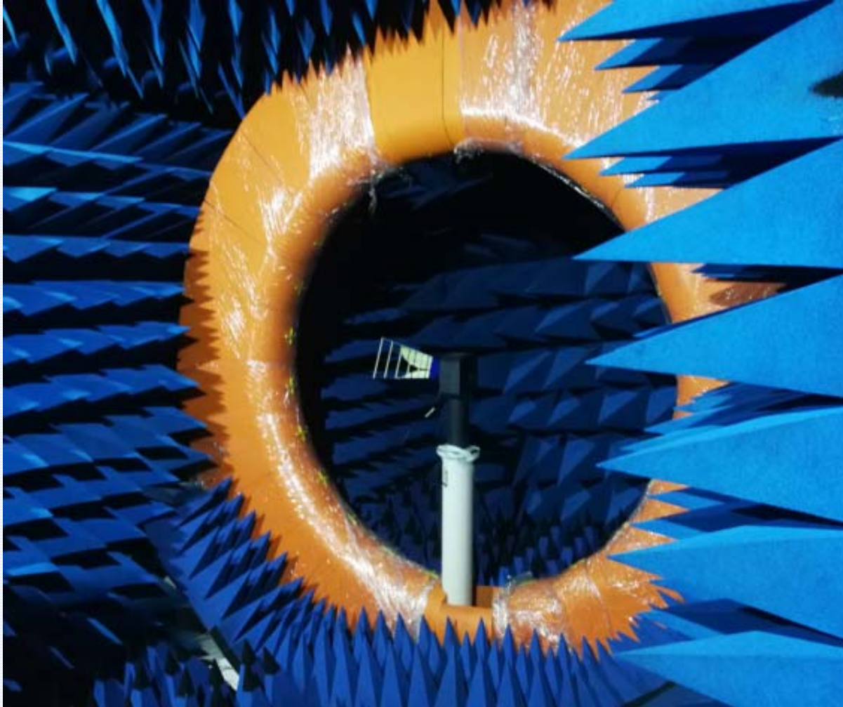
A 24-probe microwave chamber
