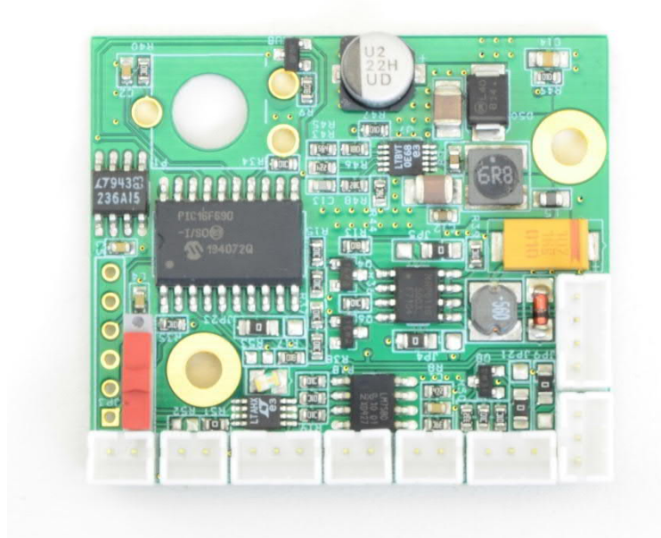
EUT_PCB brightness controller front side view (Photos provided by the applicant)
