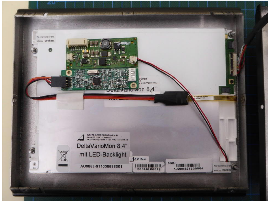
EUT Opened view 2
