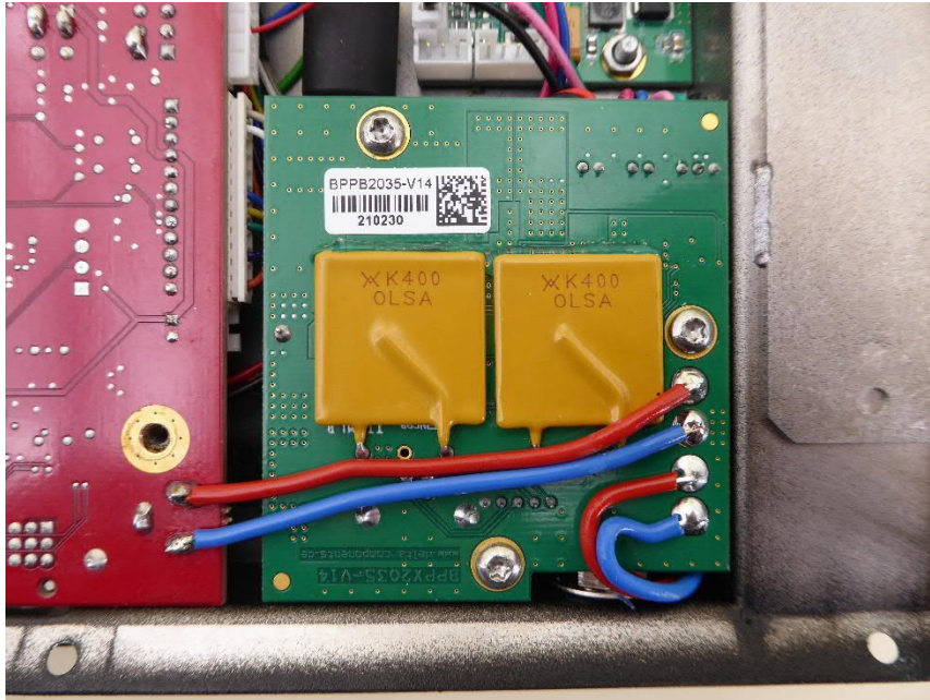
EUT Opened view 4
