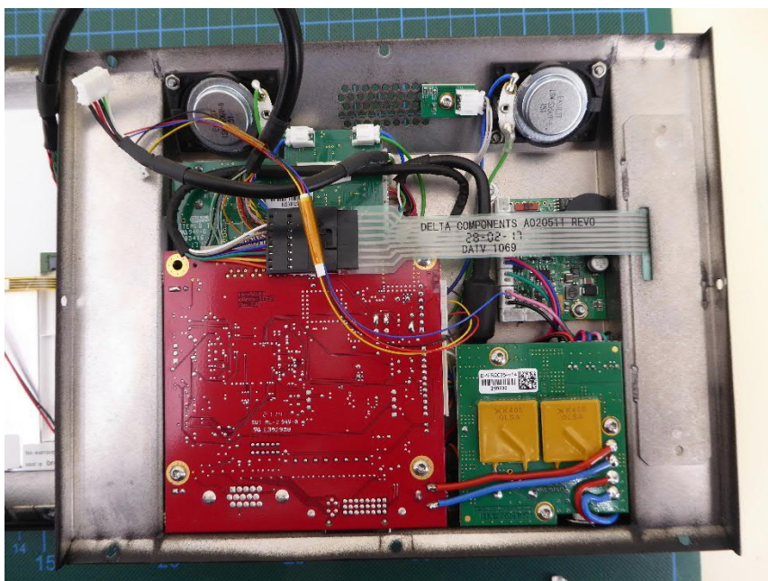
EUT Opened view 1
