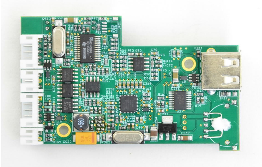
EUT_PCB USB-HUB & Sound front side view (Photos provided by the applicant)
