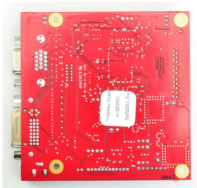
EUT_PCB graphic controller rear side view (Photos provided by the applicant)
