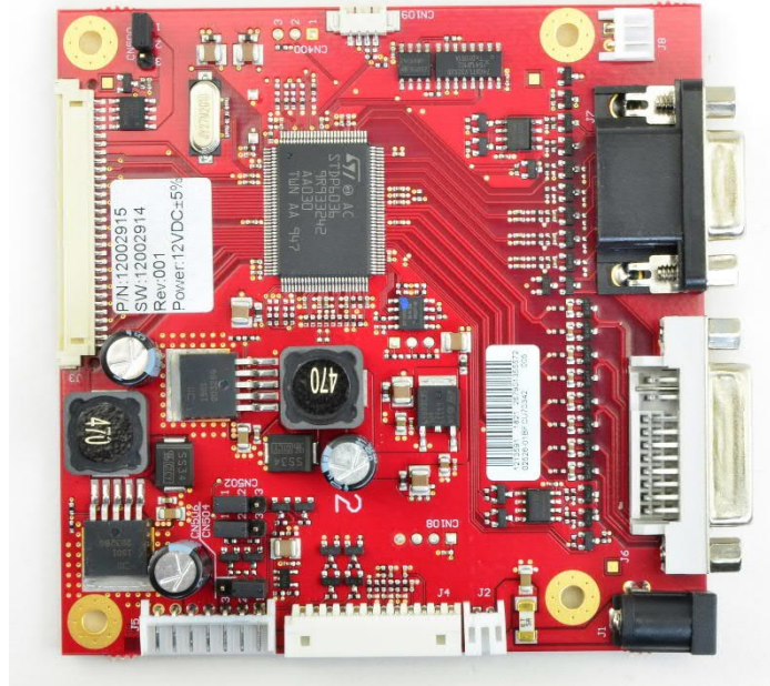
EUT_PCB graphic controller front side view (Photos provided by the applicant)
