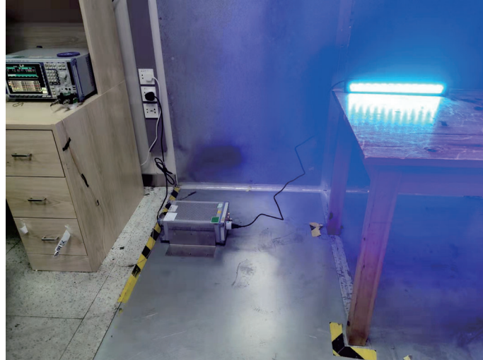
Conducted Emission
