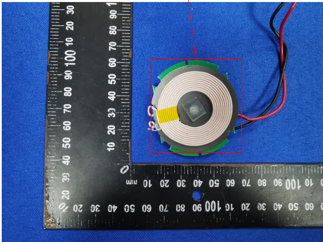
Coil antenna
