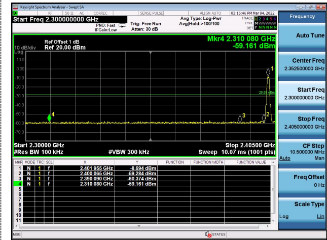
Left bandedge
