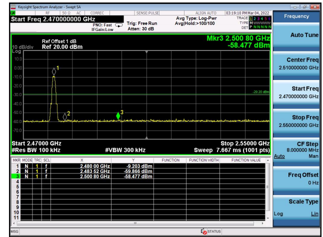
Right bandedge
