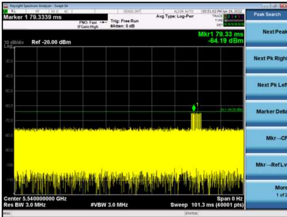
Radar Signal 2
