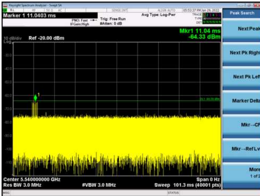
Radar Signal 6
