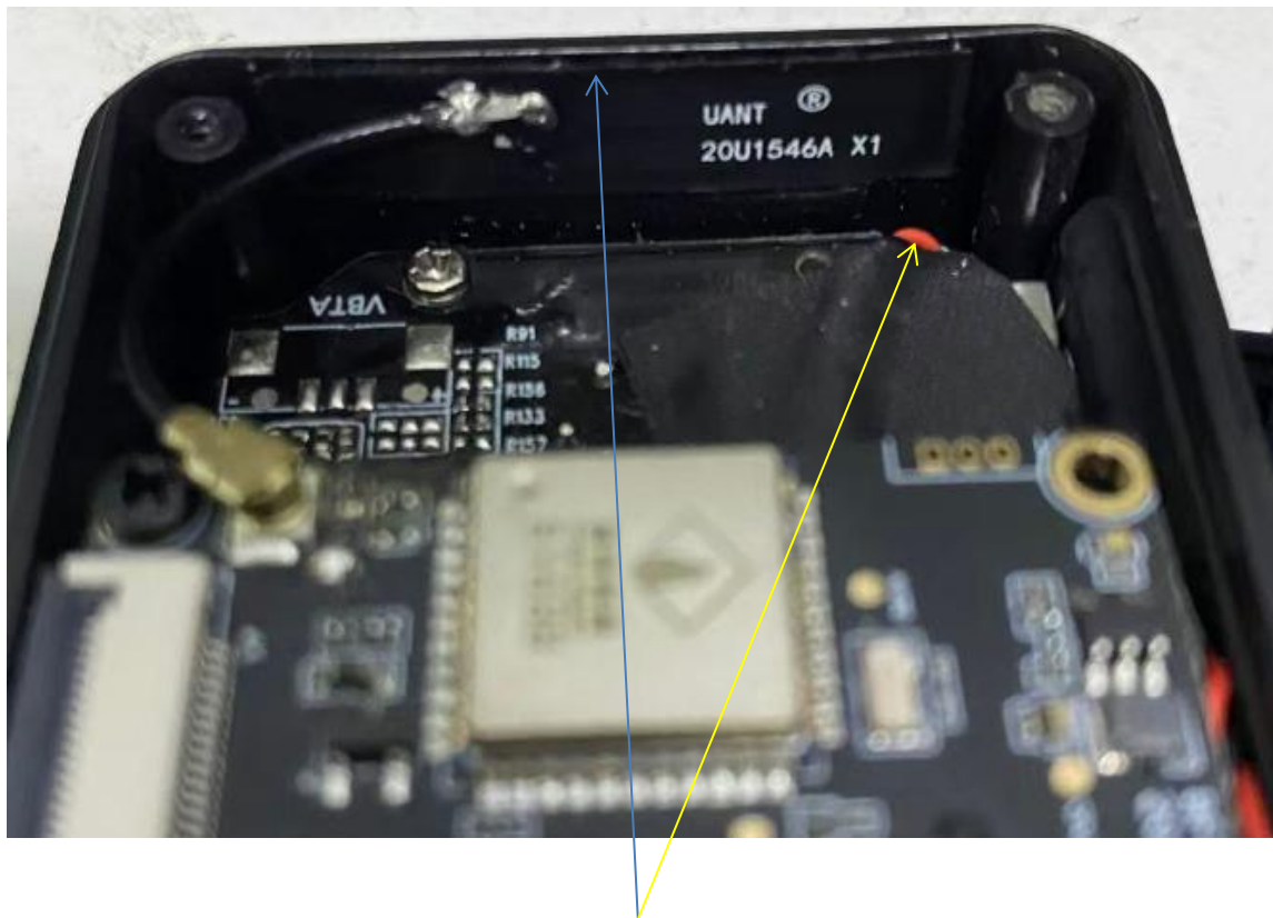
The antenna should be positioned at the center above the mounting shell, with the connecting wires attached to the board without touching the antenna.
