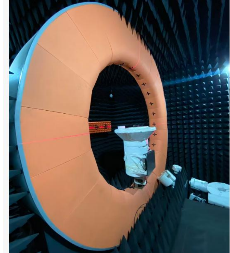
Testing 3D microwave darkroom(3m*3m*3m)
