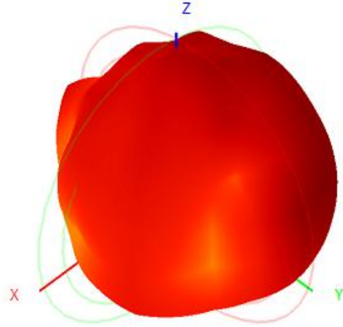
Far-field pattern
