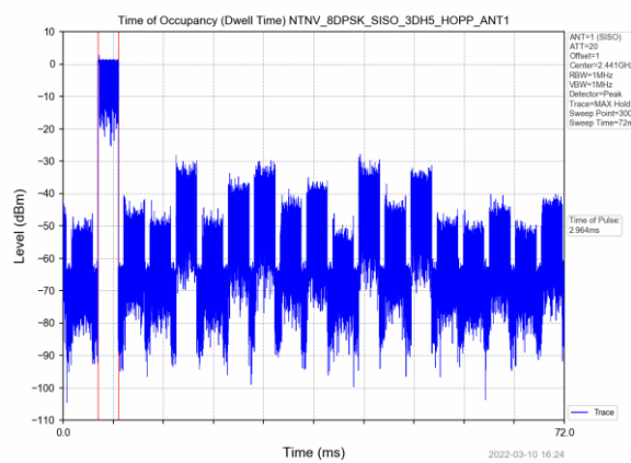
3DH5
