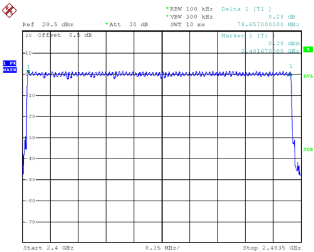
Modulation: 8DPSK
