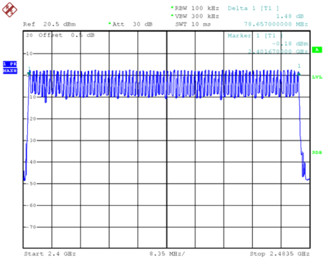
Modulation: GFSK
