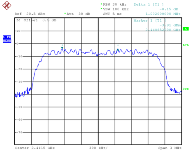
Middle Channel
