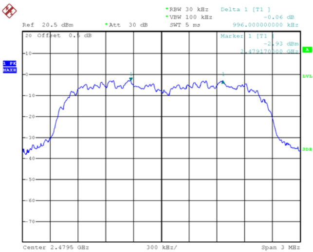
High Channel
