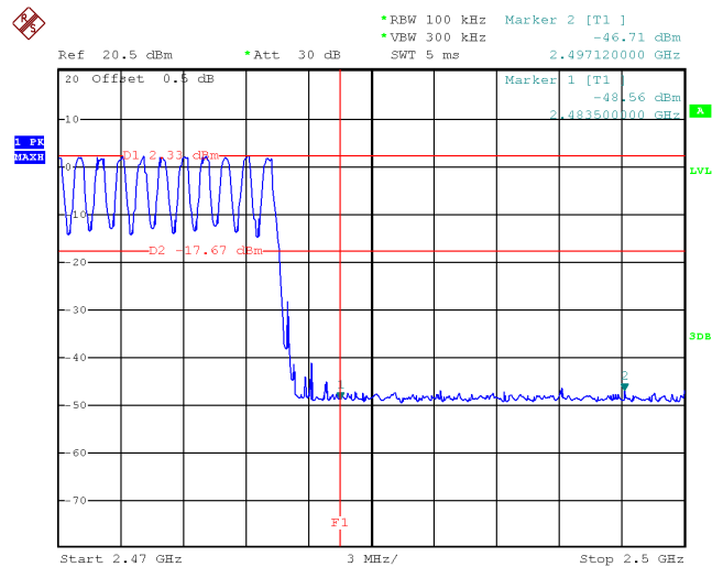
Hopping Band edge-right side
