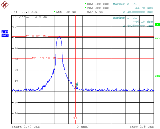
Transmitting Band edge-right side
