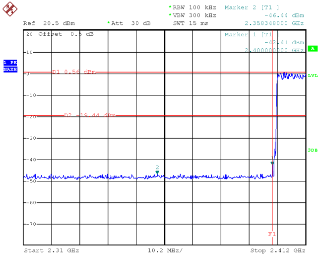
Hopping Band edge-left side
