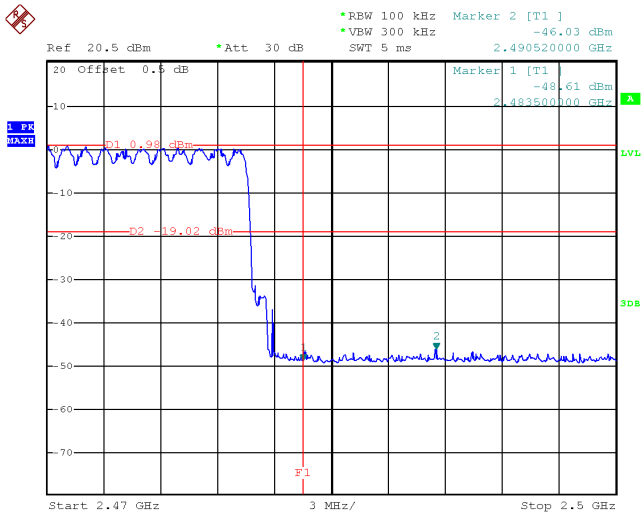
Hopping Band edge-right side
