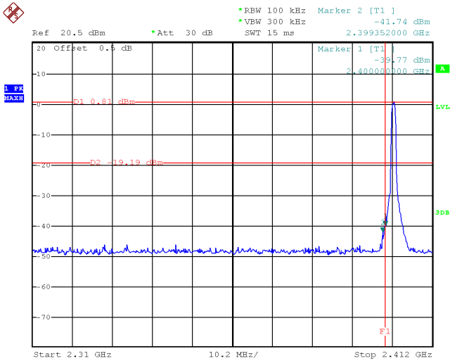
Transmitting Band edge-left side
