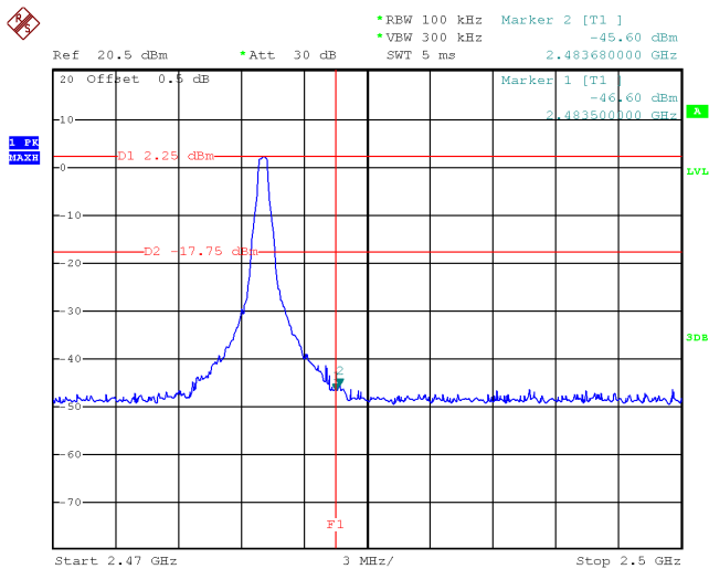
Transmitting Band edge-right side
