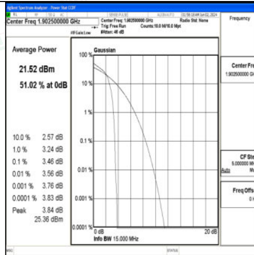
Band2-15MHz-16QAM-19125-1RB#0-PASS
