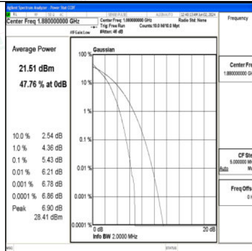
Band2-1.4MHz-QPSK-18900-6RB#0-PASS
