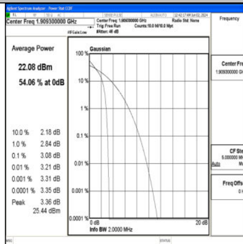
Band2-1.4MHz-QPSK-19193-1RB#0-PASS
