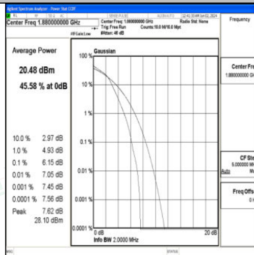
Band2-1.4MHz-16QAM-18900-6RB#0-PASS
