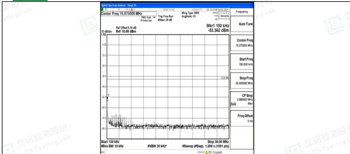
Band2_5MHz_16QAM_18900_1RB#0_0.15~30_0.15~30
