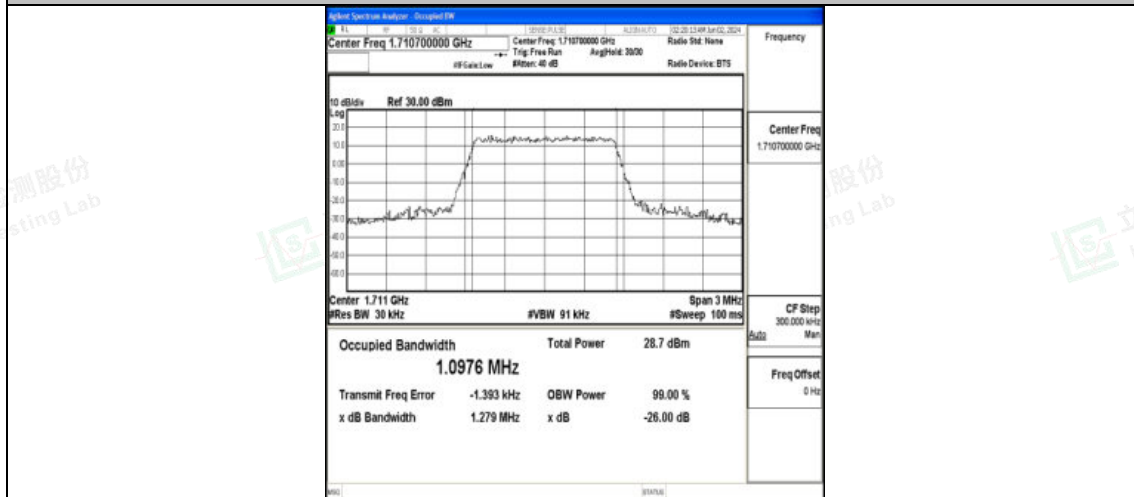
Band4-1.4MHz-16QAM-19957-6RB#0-PASS
