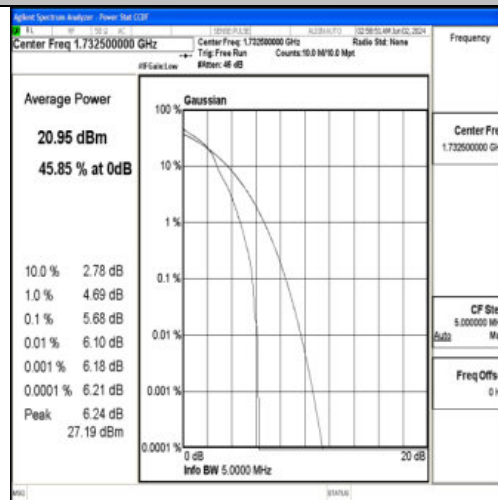
Band4-3MHz-16QAM-20175-1RB#0-PASS
