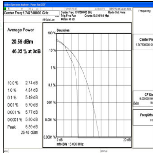
Band4-15MHz-16QAM-20325-1RB#0-PASS
