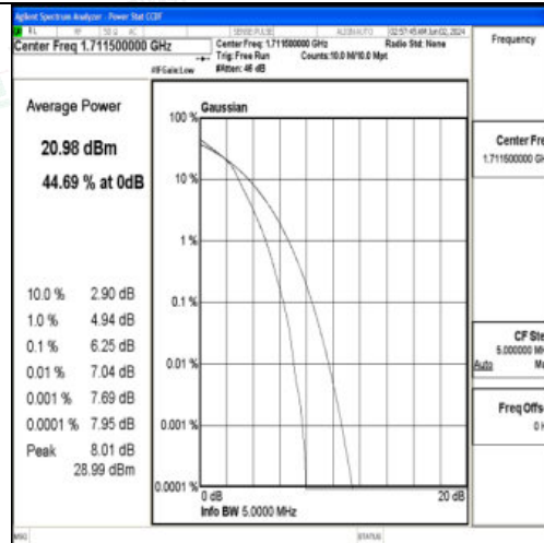
Band4-3MHz-16QAM-19965-15RB#0-PASS
