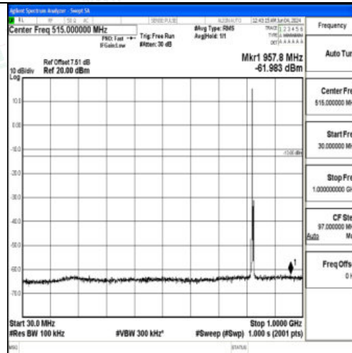
Band5_3MHz_QPSK_20415_1RB#0_30~1000_30~1000
