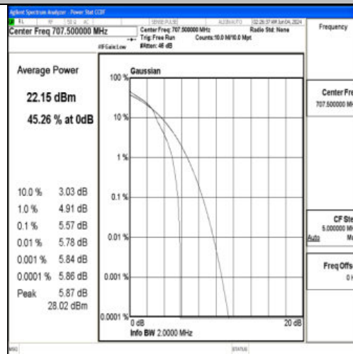
Band12-1.4MHz-16QAM-23095-1RB#0-PASS
