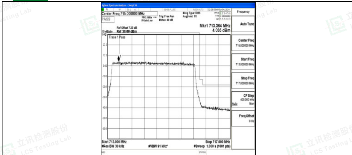
Band12_3MHz_16QAM_23165_15RB#0
