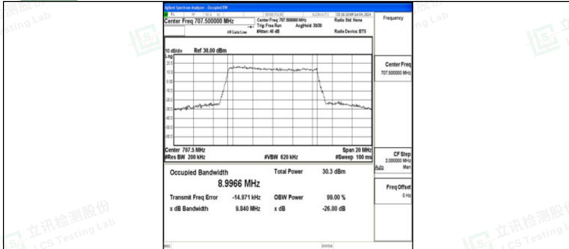
Band12-10MHz-16QAM-23095-50RB#0-PASS
