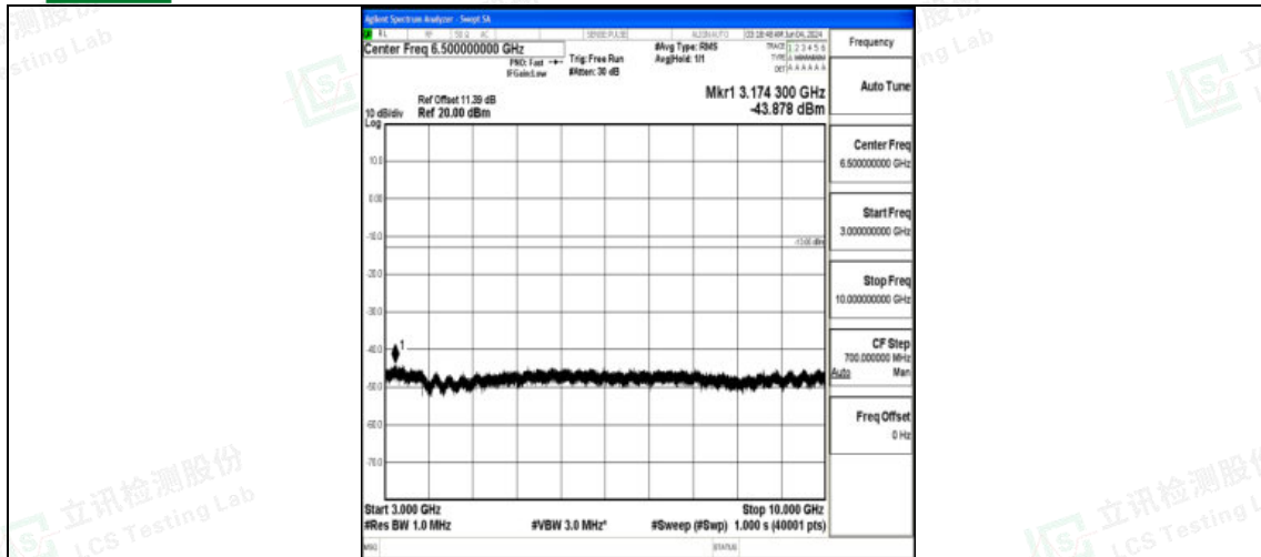
Band12_10MHz_QPSK_23095_1RB#0_3000~10000_3000~10000
