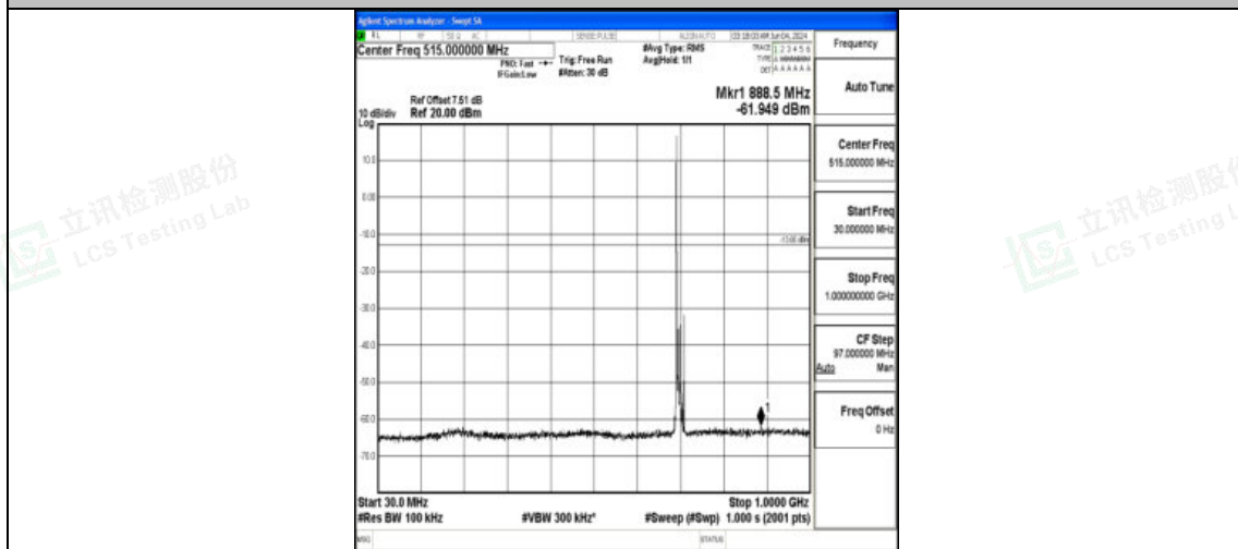
Band12_10MHz_16QAM_23060_1RB#0_30~1000_30~1000
