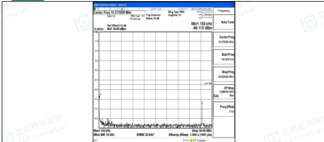
Band41_10MHz_QPSK_40620_1RB#0_0.15~30_0.15~30
