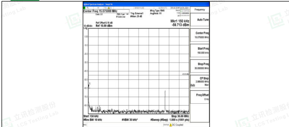
Band41_20MHz_QPSK_40620_1RB#0_0.15~30_0.15~30
