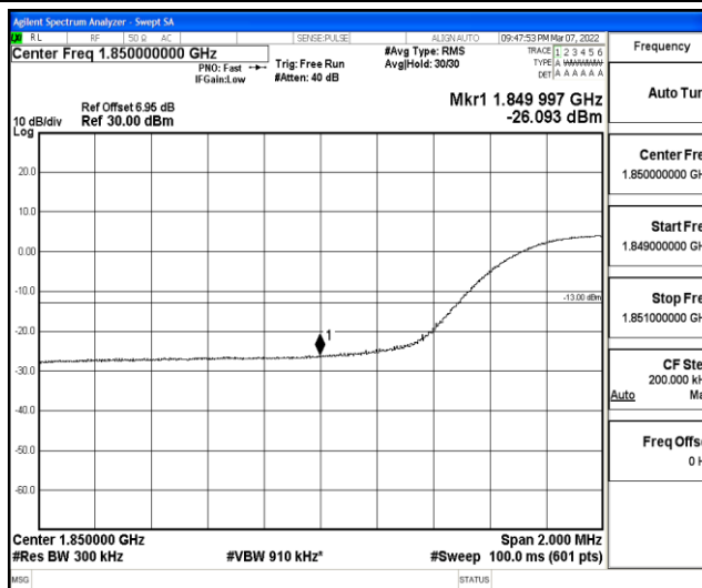
Band2-15MHz-QPSK-19125-75RB#0
