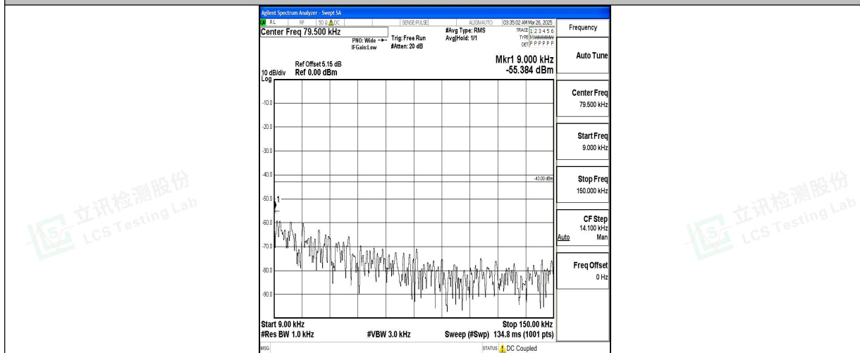
Band2_20MHz_QPSK_18700_1RB#0_0.009~0.15_0.009~0.15
