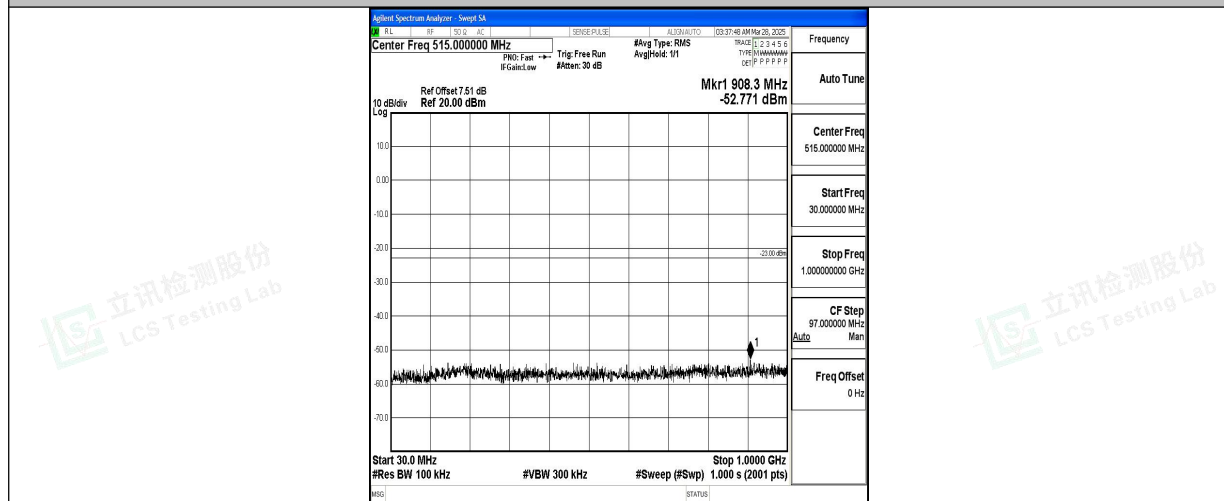
Band2_20MHz_16QAM_19100_1RB#0_30~1000_30~1000
