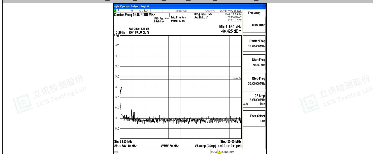
Band2_20MHz_16QAM_18700_1RB#0_0.15~30_0.15~30
