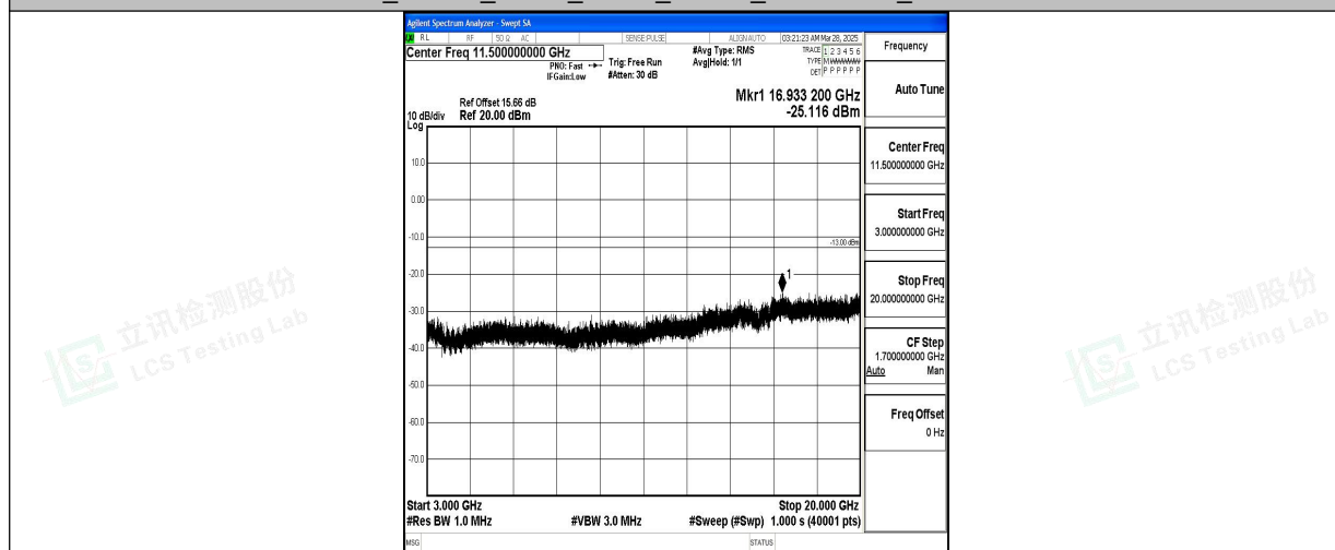
Band2_15MHz_QPSK_19125_1RB#0_3000~20000_3000~20000
