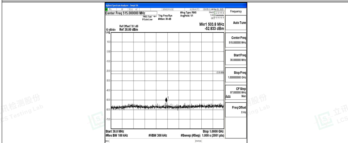
Band2_20MHz_QPSK_18700_1RB#0_30~1000_30~1000
