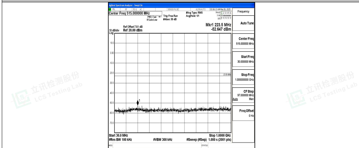
Band2_20MHz_QPSK_18900_1RB#0_30~1000_30~1000
