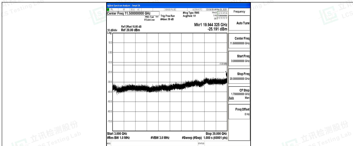
Band2_20MHz_16QAM_18900_1RB#0_3000~20000_3000~20000
