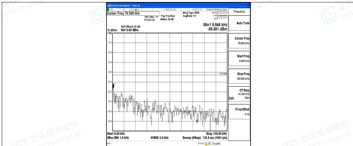
Band2_20MHz_QPSK_18900_1RB#0_0.009~0.15_0.009~0.15
