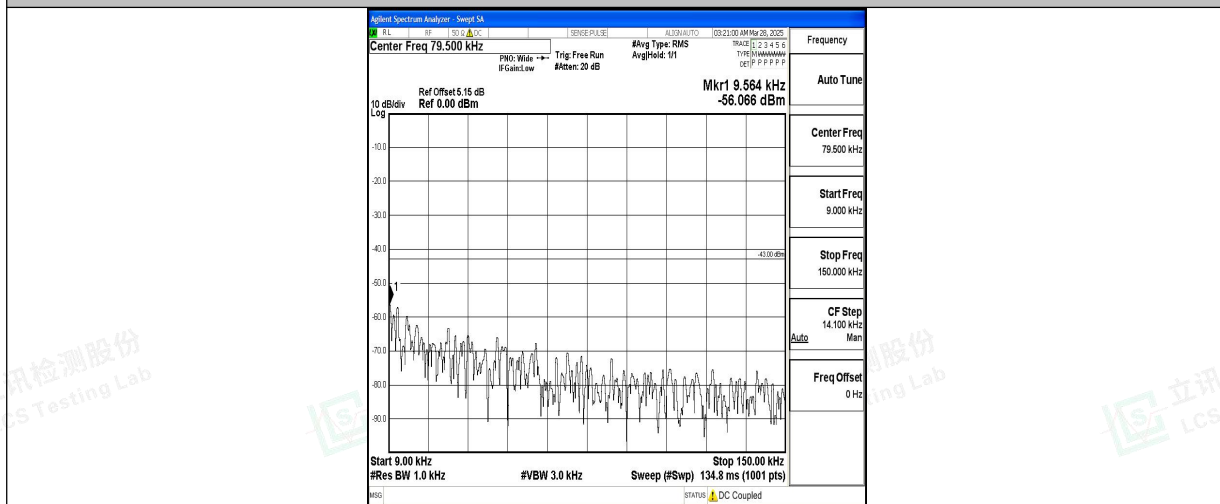
Band2_15MHz_QPSK_19125_1RB#0_0.009~0.15_0.009~0.15
