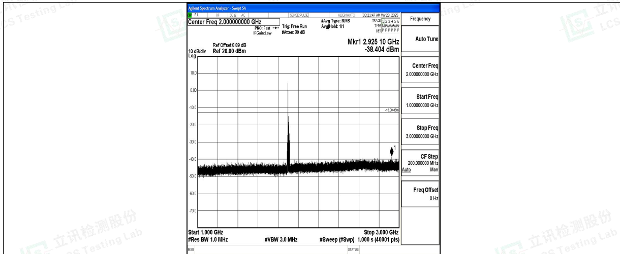
Band2_15MHz_16QAM_19125_1RB#0_1000~3000_1000~3000
