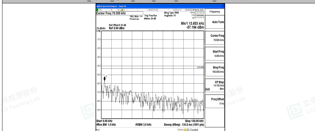
Band2_20MHz_16QAM_18700_1RB#0_0.009~0.15_0.009~0.15
