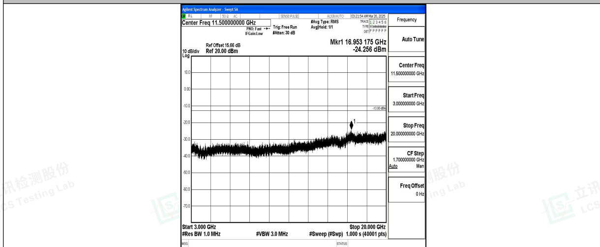
Band2_15MHz_16QAM_19125_1RB#0_3000~20000_3000~20000
