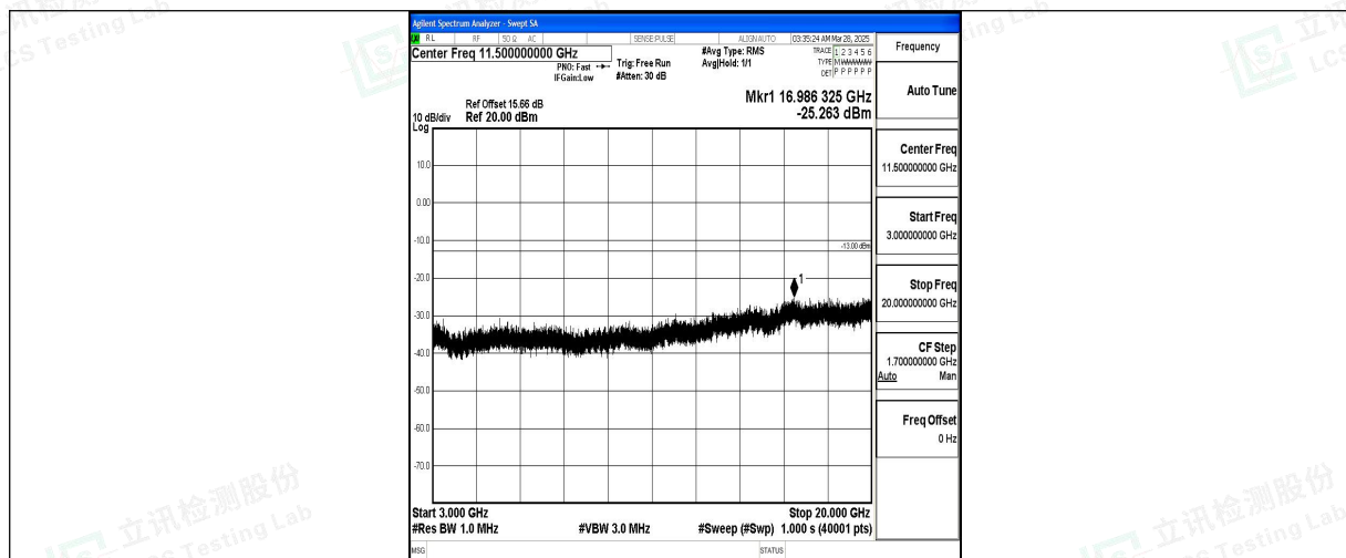
Band2_20MHz_QPSK_18700_1RB#0_3000~20000_3000~20000
