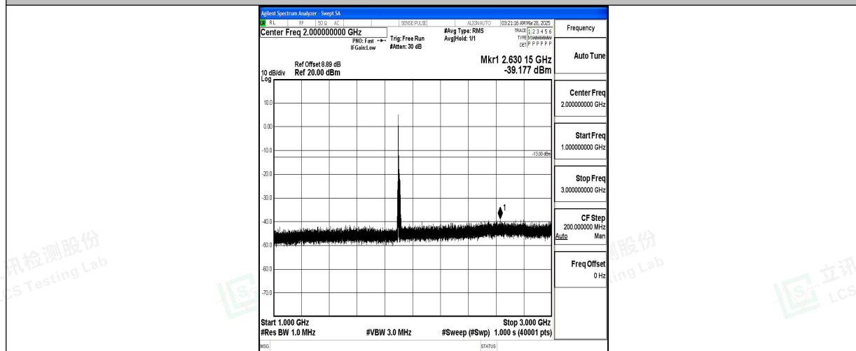
Band2_15MHz_QPSK_19125_1RB#0_1000~3000_1000~3000
