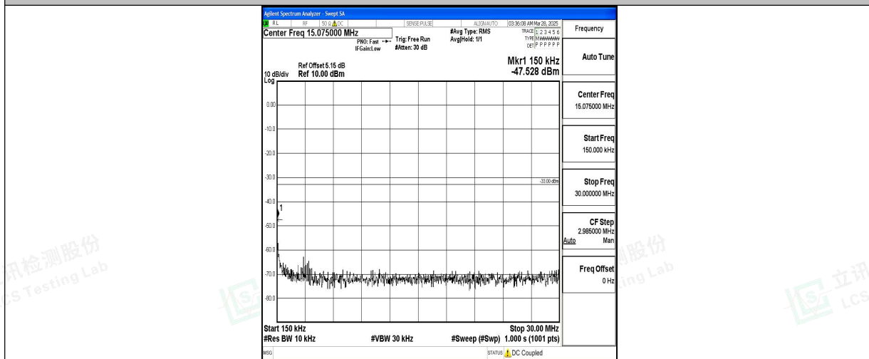
Band2_20MHz_QPSK_18900_1RB#0_0.15~30_0.15~30
