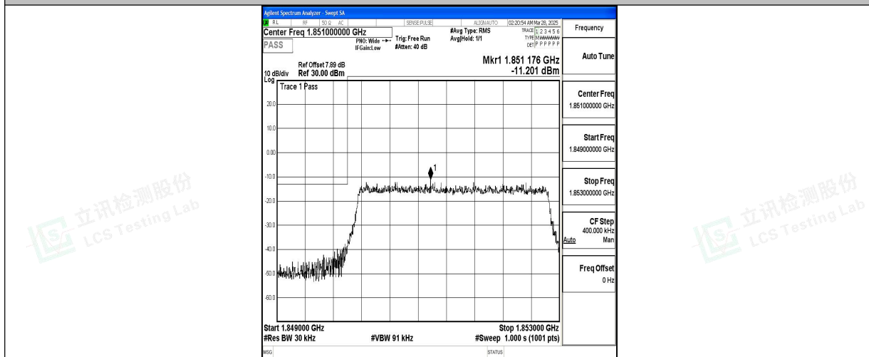
Band2_3MHz_16QAM_18615_15RB#0
