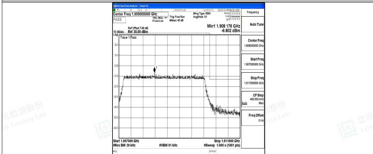
Band2_3MHz_16QAM_19185_15RB#0
