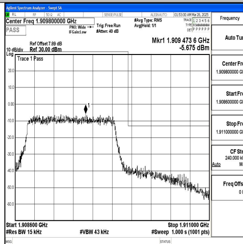
Band2_1.4MHz_QPSK_19193_6RB#0
