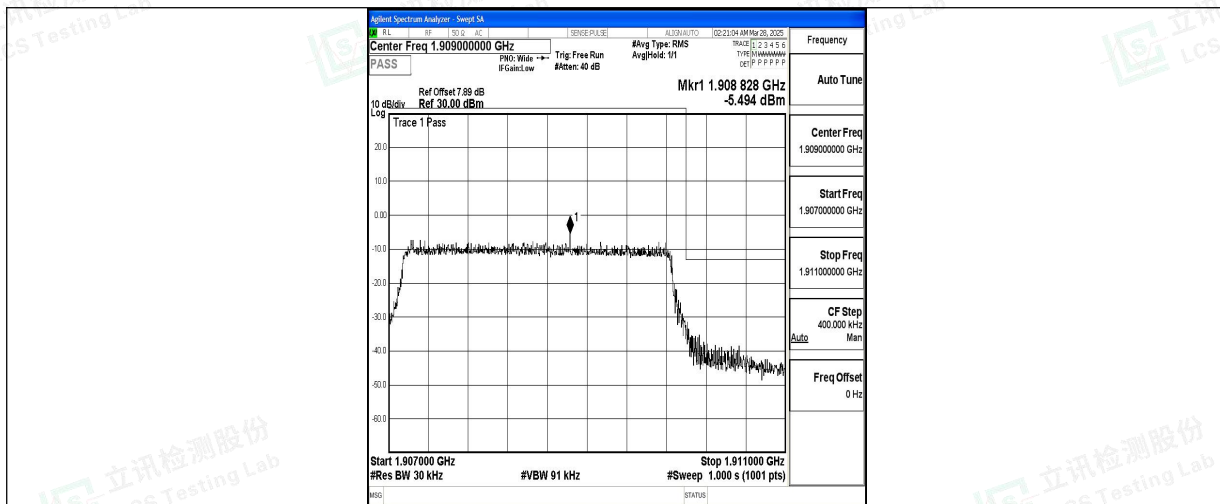
Band2_3MHz_QPSK_19185_15RB#0
