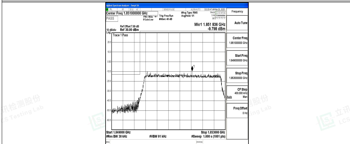
Band2_3MHz_QPSK_18615_15RB#0
