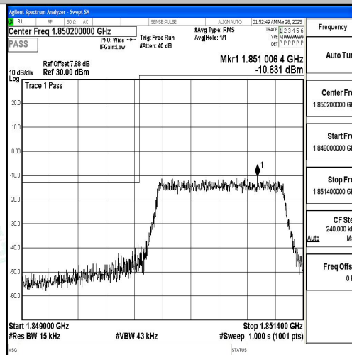
Band2_1.4MHz_16QAM_18607_6RB#0
