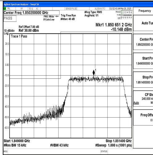
Band2_1.4MHz_QPSK_18607_6RB#0
