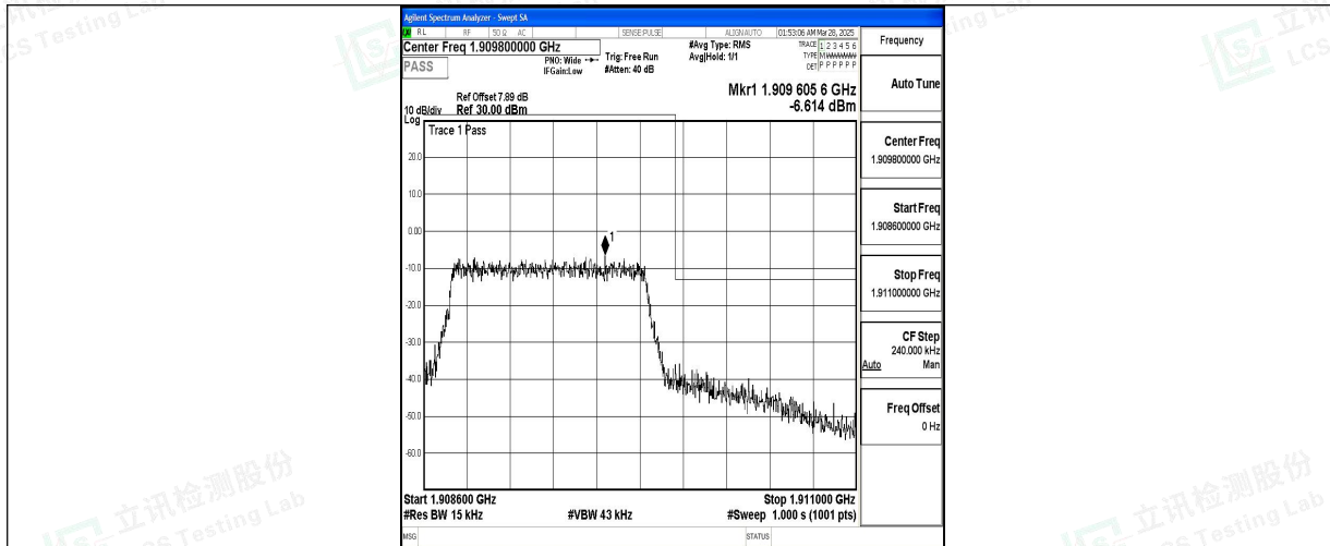
Band2_1.4MHz_16QAM_19193_6RB#0
