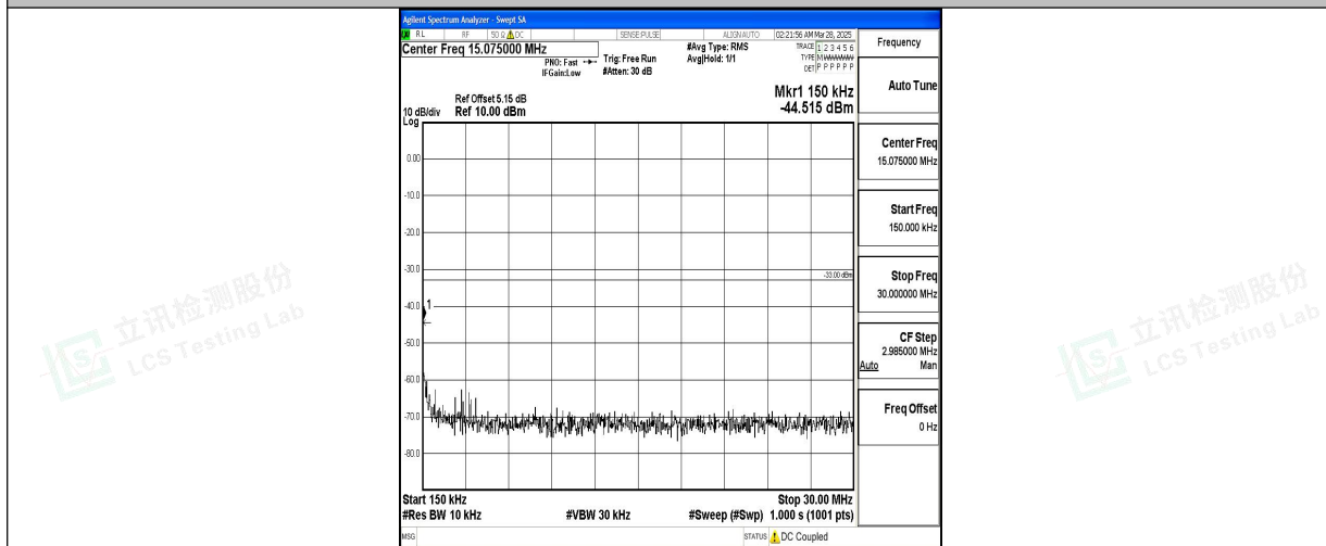
Band2_3MHz_16QAM_18615_1RB#0_0.15~30_0.15~30
