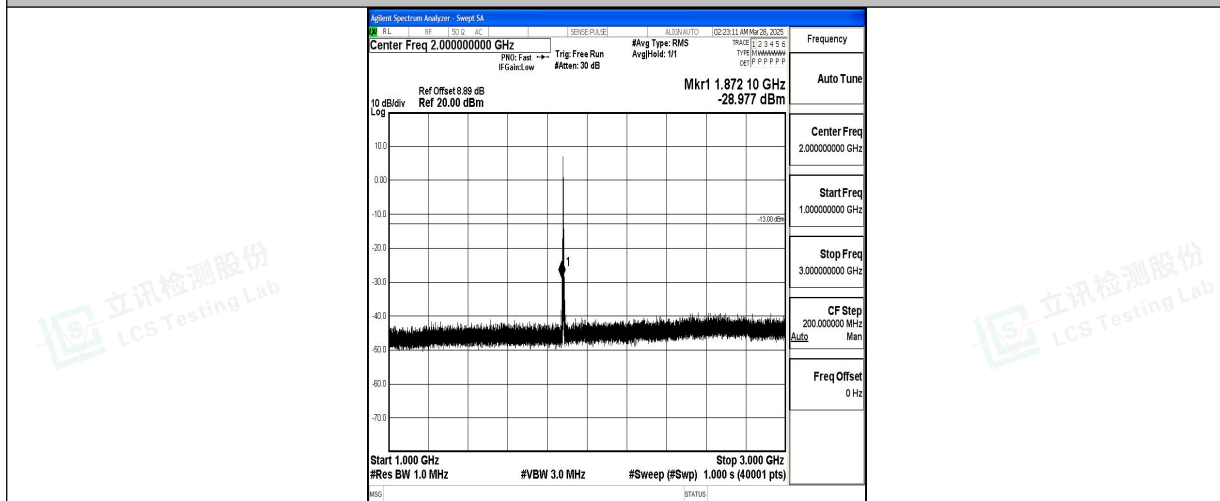
Band2_3MHz_16QAM_18900_1RB#0_1000~3000_1000~3000
