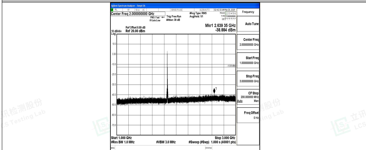
Band2_5MHz_16QAM_18625_1RB#0_1000~3000_1000~3000
