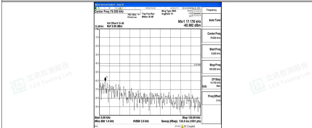
Band2_5MHz_QPSK_18625_1RB#0_0.009~0.15_0.009~0.15
