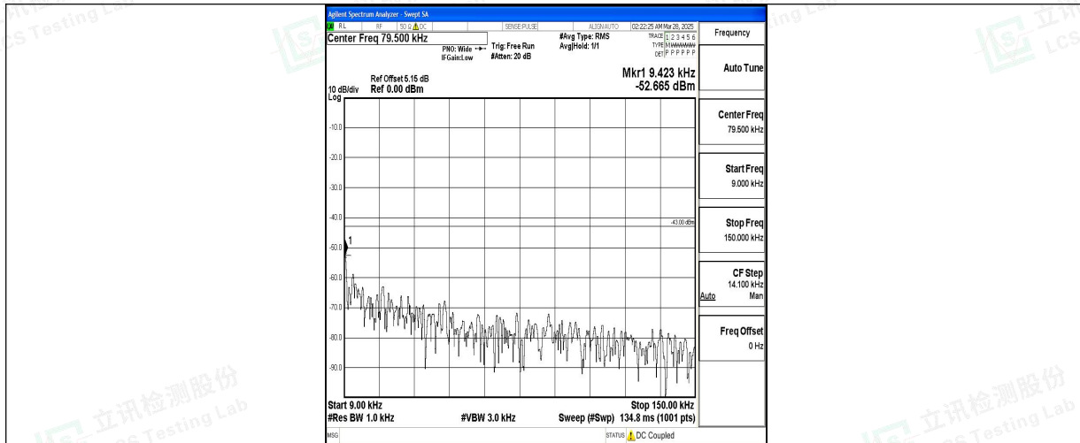
Band2_3MHz_QPSK_18900_1RB#0_0.009~0.15_0.009~0.15
