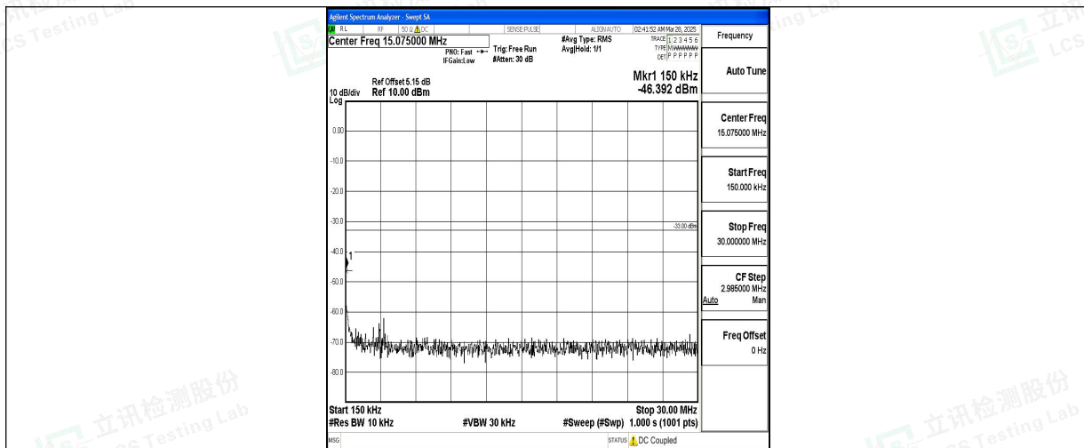
Band2_5MHz_QPSK_18625_1RB#0_0.15~30_0.15~30
