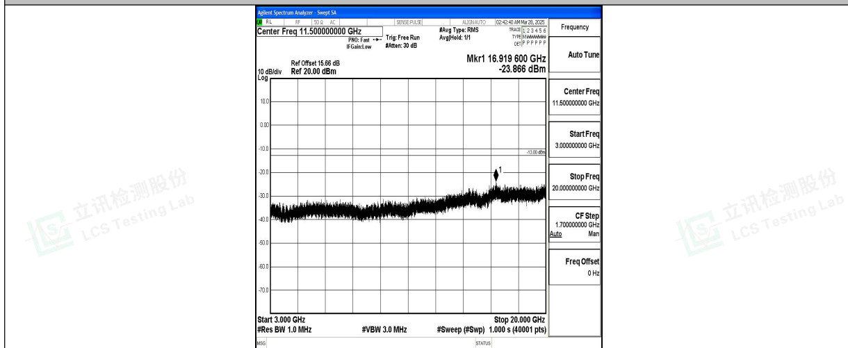
Band2_5MHz_16QAM_18625_1RB#0_3000~20000_3000~20000
