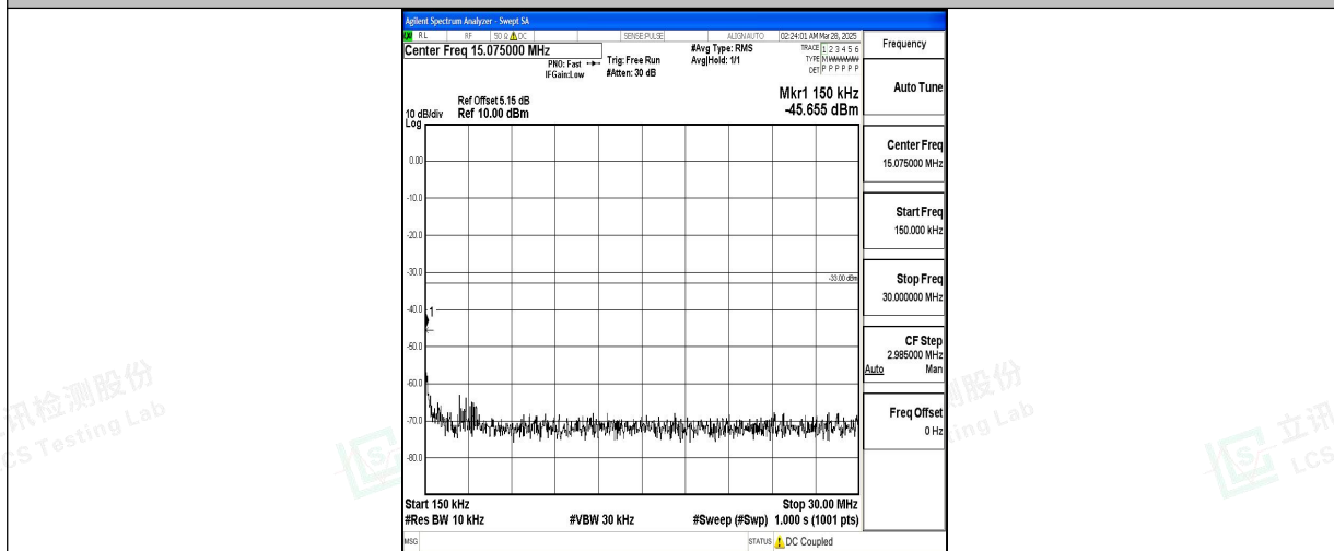
Band2_3MHz_16QAM_19185_1RB#0_0.15~30_0.15~30
