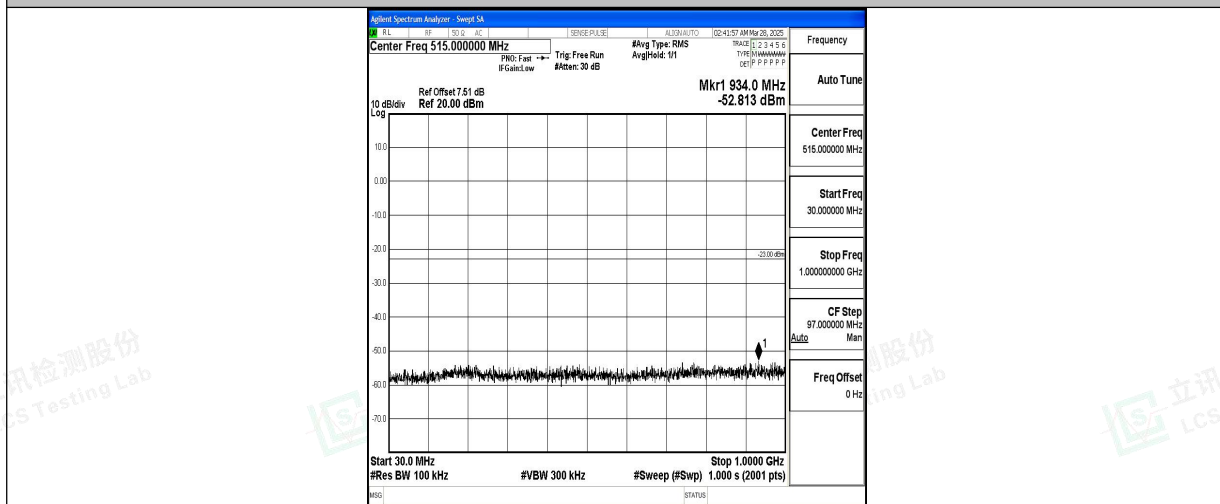
Band2_5MHz_QPSK_18625_1RB#0_30~1000_30~1000
