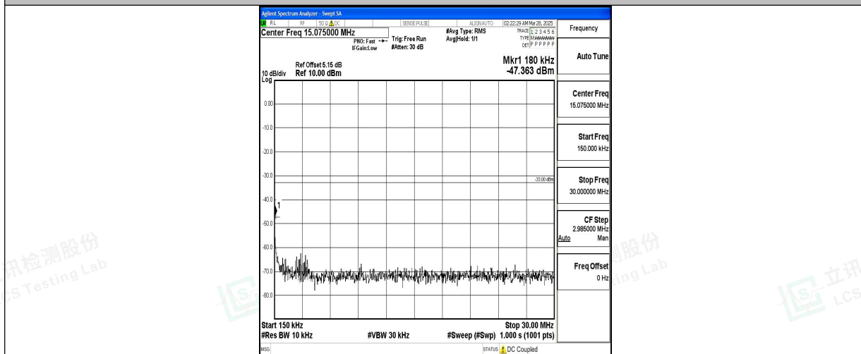
Band2_3MHz_QPSK_18900_1RB#0_0.15~30_0.15~30
