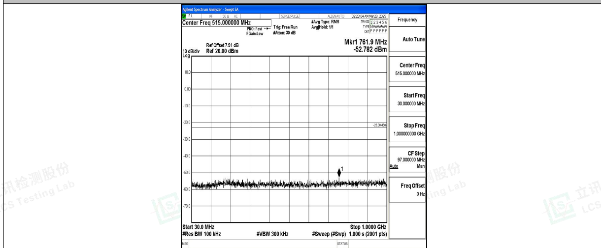
Band2_3MHz_16QAM_18900_1RB#0_30~1000_30~1000
