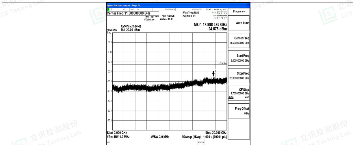
Band2_5MHz_QPSK_18625_1RB#0_3000~20000_3000~20000
