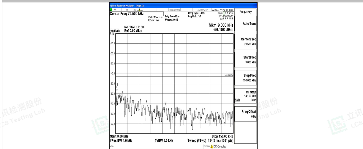
Band2_5MHz_16QAM_18625_1RB#0_0.009~0.15_0.009~0.15
