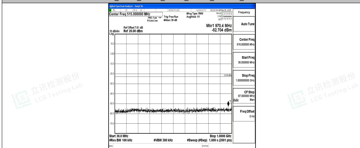
Band2_3MHz_QPSK_18900_1RB#0_30~1000_30~1000
