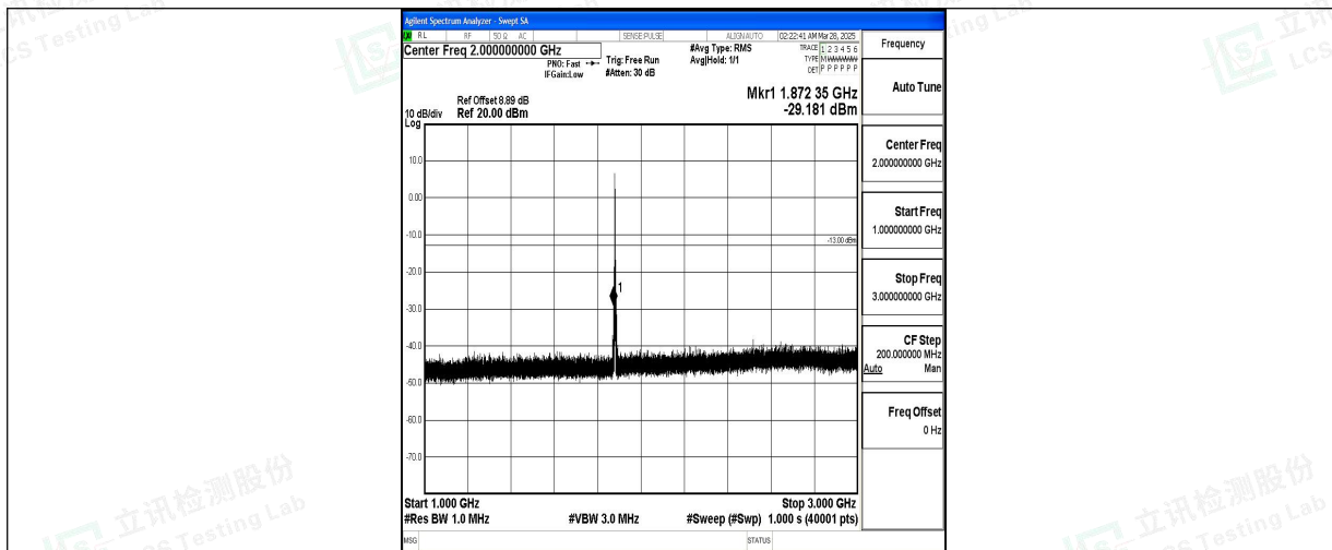
Band2_3MHz_QPSK_18900_1RB#0_1000~3000_1000~3000
