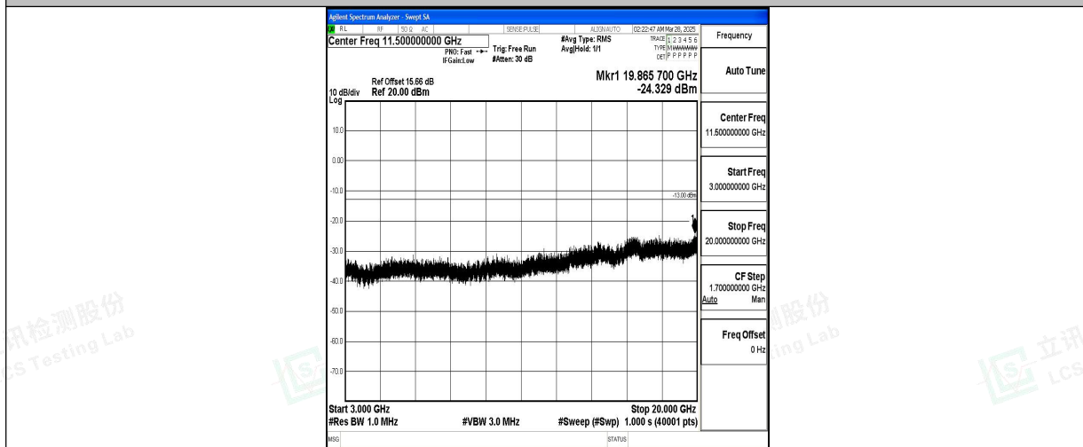
Band2_3MHz_QPSK_18900_1RB#0_3000~20000_3000~20000
