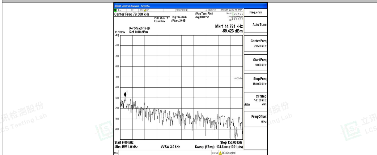
Band2_3MHz_QPSK_19185_1RB#0_0.009~0.15_0.009~0.15
