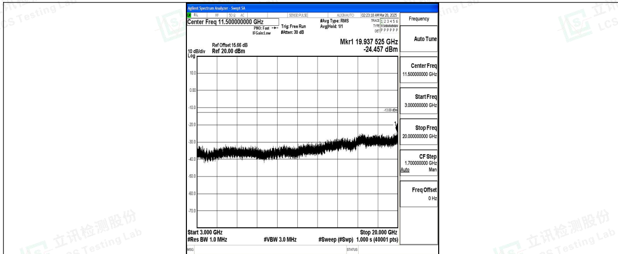
Band2_3MHz_16QAM_18900_1RB#0_3000~20000_3000~20000
