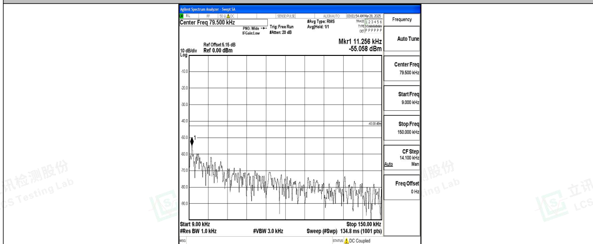
Band2_10MHz_16QAM_18650_1RB#0_0.009~0.15_0.009~0.15
