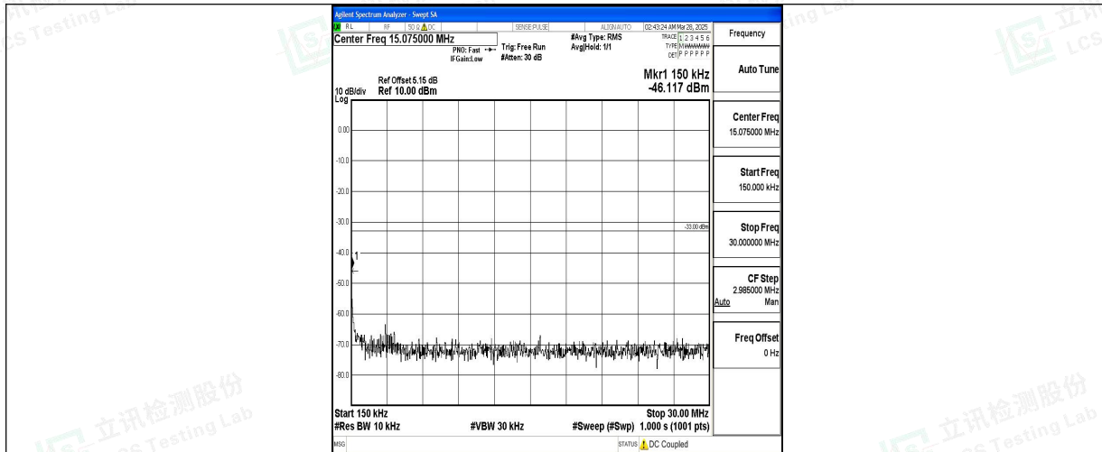
Band2_5MHz_16QAM_18900_1RB#0_0.15~30_0.15~30
