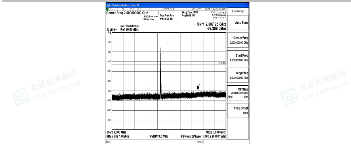
Band2_10MHz_QPSK_18650_1RB#0_1000~3000_1000~3000
