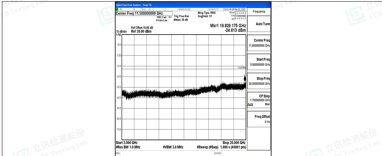
Band2_10MHz_QPSK_18650_1RB#0_3000~20000_3000~20000
