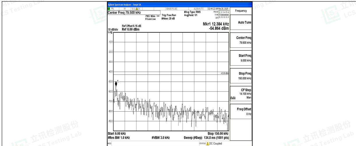
Band2_5MHz_16QAM_19175_1RB#0_0.009~0.15_0.009~0.15
