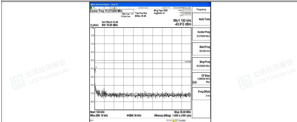
Band2_15MHz_16QAM_18675_1RB#0_0.15~30_0.15~30
