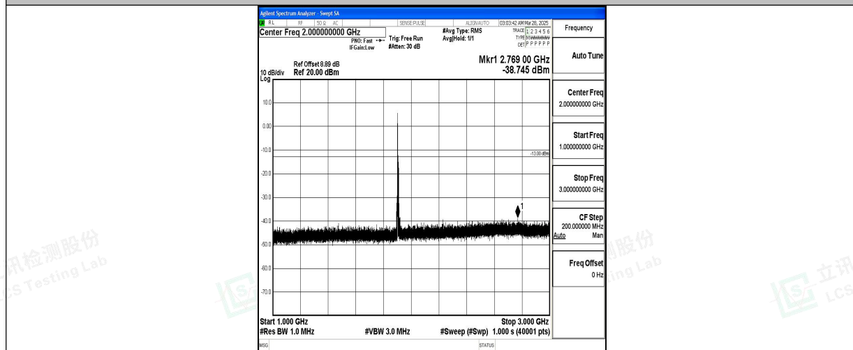
Band2_10MHz_QPSK_19150_1RB#0_1000~3000_1000~3000
