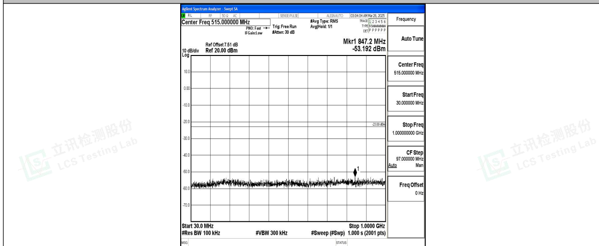
Band2_10MHz_16QAM_19150_1RB#0_30~1000_30~1000
