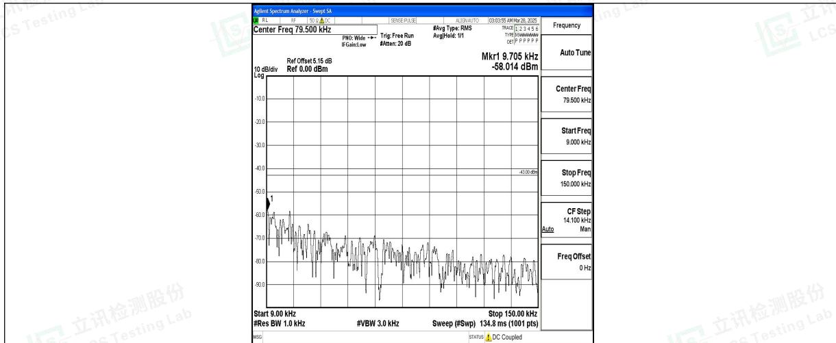
Band2_10MHz_16QAM_19150_1RB#0_0.009~0.15_0.009~0.15
