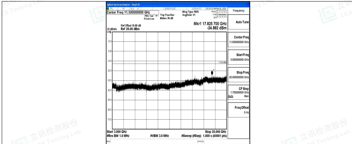
Band2_15MHz_QPSK_18675_1RB#0_3000~20000_3000~20000
