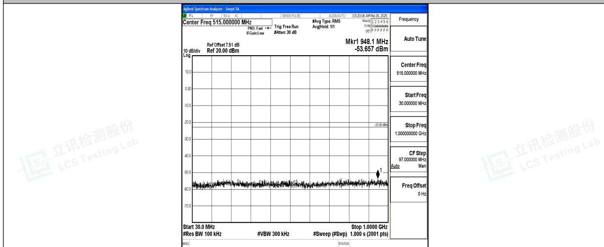
Band2_15MHz_QPSK_18900_1RB#0_30~1000_30~1000
