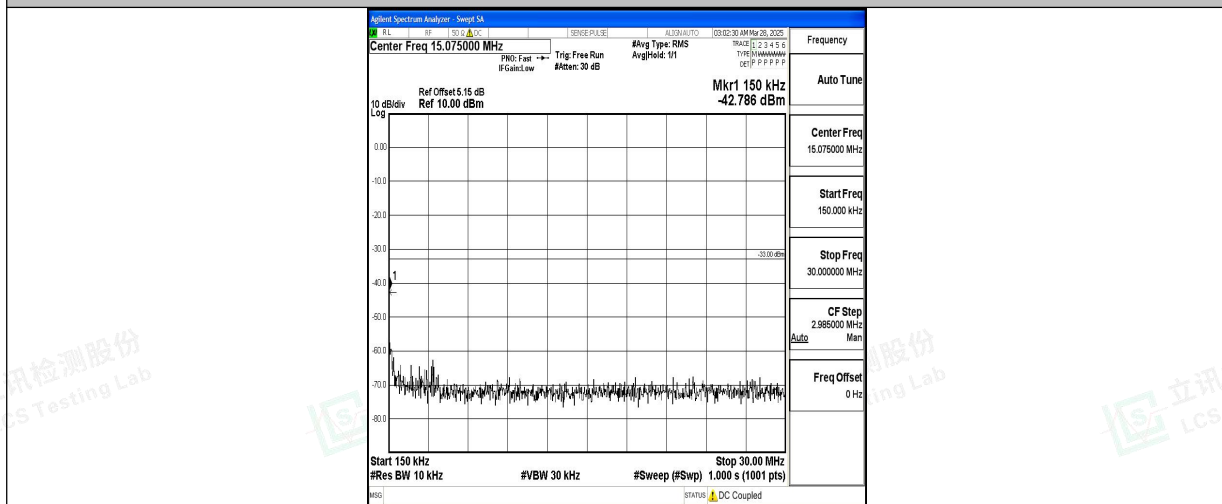
Band2_10MHz_QPSK_18900_1RB#0_0.15~30_0.15~30
