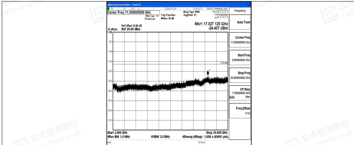
Band2_10MHz_16QAM_18900_1RB#0_3000~20000_3000~20000
