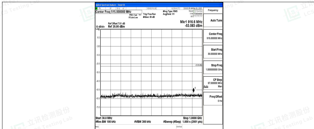
Band2_10MHz_QPSK_19150_1RB#0_30~1000_30~1000
