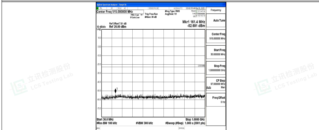
Band2_10MHz_QPSK_18900_1RB#0_30~1000_30~1000
