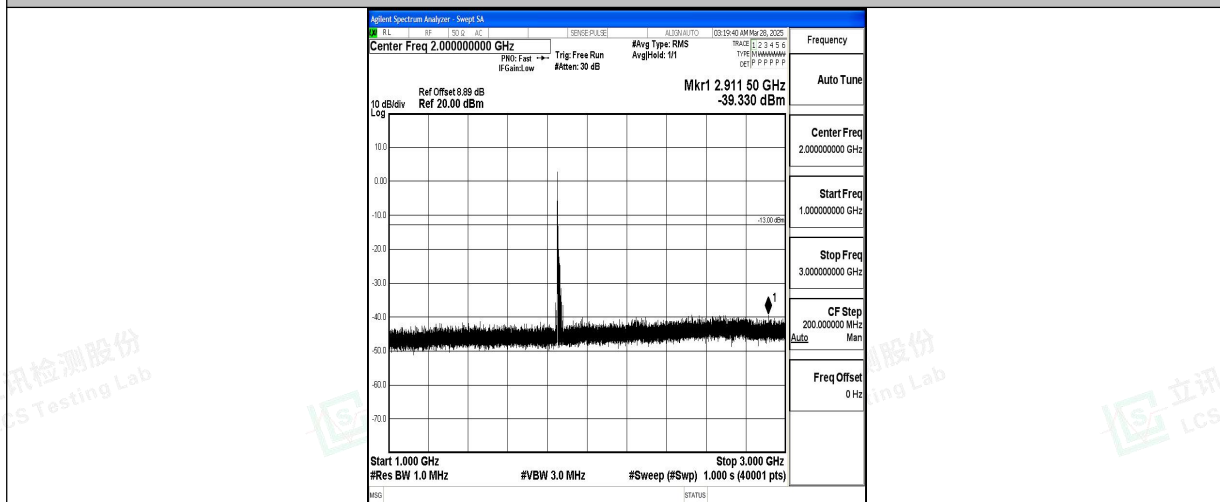
Band2_15MHz_16QAM_18675_1RB#0_1000~3000_1000~3000
