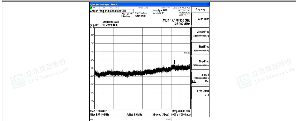
Band4_15MHz_QPSK_20025_1RB#0_3000~20000_3000~20000
