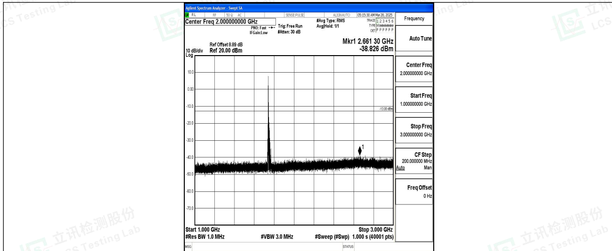
Band4_15MHz_QPSK_20325_1RB#0_1000~3000_1000~3000
