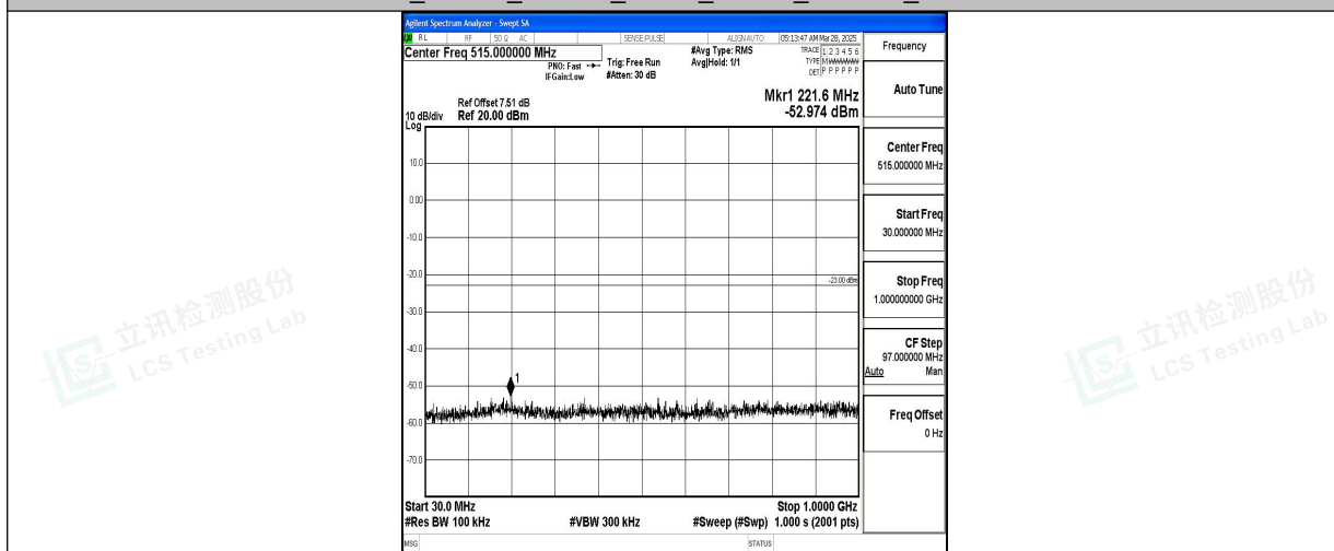
Band4_15MHz_16QAM_20025_1RB#0_30~1000_30~1000
