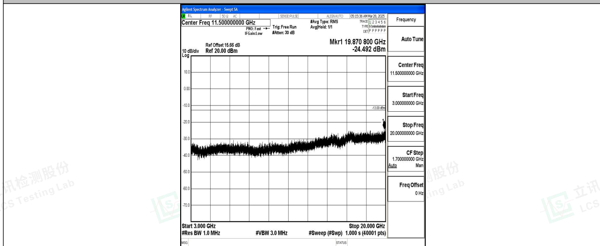
Band4_15MHz_QPSK_20325_1RB#0_3000~20000_3000~20000
