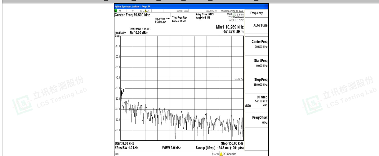
Band4_15MHz_16QAM_20325_1RB#0_0.009~0.15_0.009~0.15
