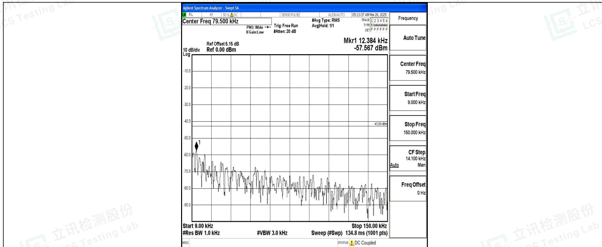
Band4_15MHz_16QAM_20025_1RB#0_0.009~0.15_0.009~0.15
