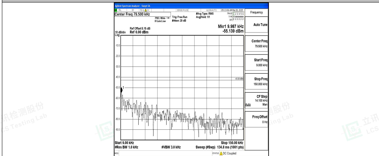
Band4_15MHz_QPSK_20025_1RB#0_0.009~0.15_0.009~0.15
