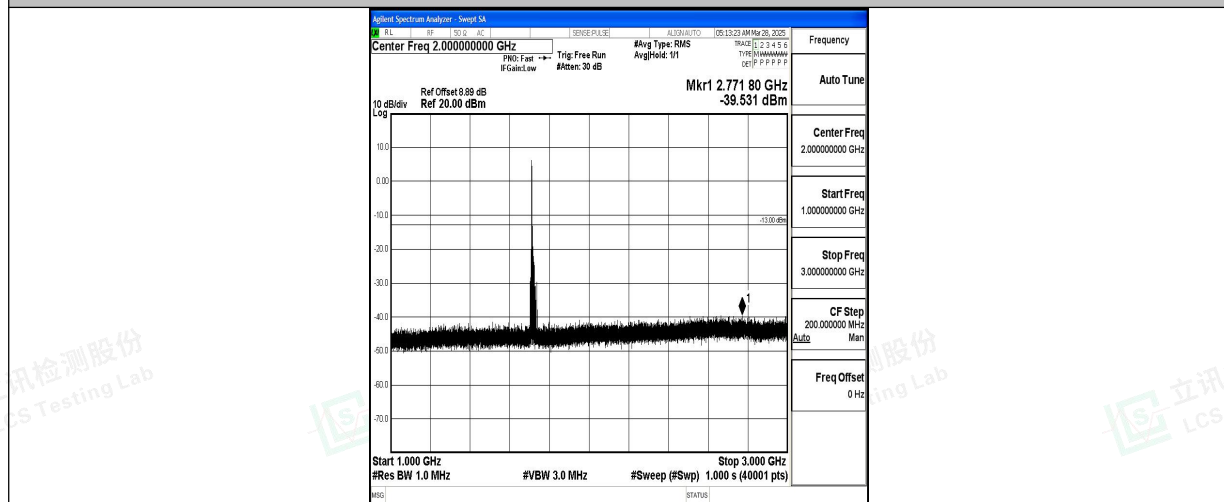
Band4_15MHz_QPSK_20025_1RB#0_1000~3000_1000~3000
