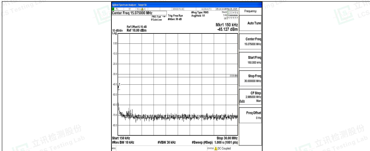
Band4_15MHz_QPSK_20175_1RB#0_0.15~30_0.15~30
