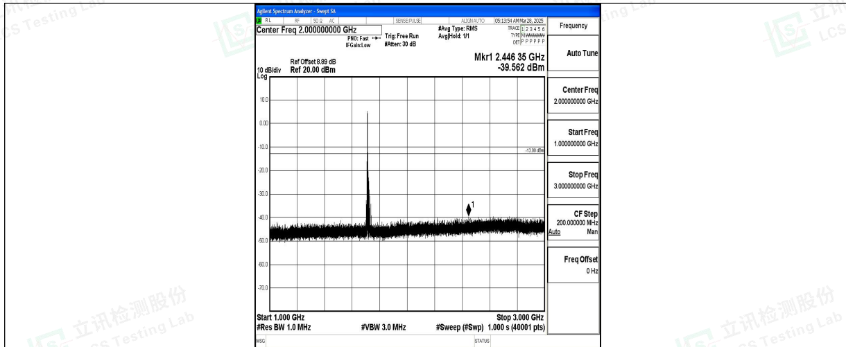
Band4_15MHz_16QAM_20025_1RB#0_1000~3000_1000~3000
