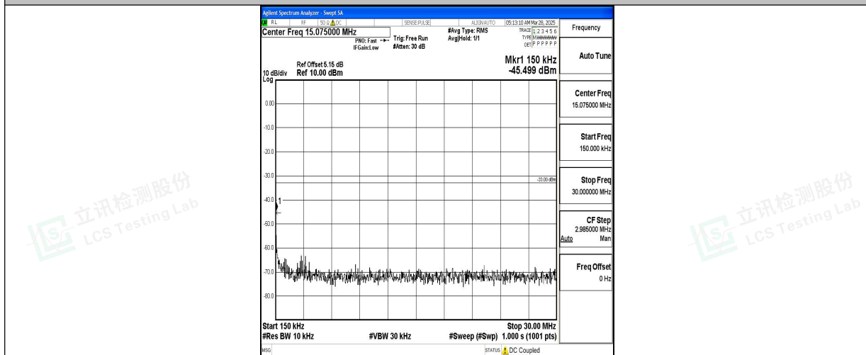
Band4_15MHz_QPSK_20025_1RB#0_0.15~30_0.15~30
