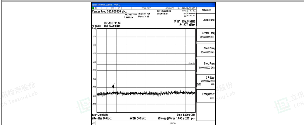
Band4_15MHz_QPSK_20175_1RB#0_30~1000_30~1000
