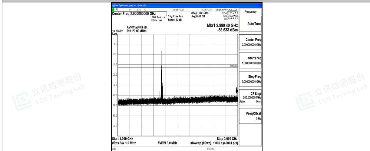
Band4_15MHz_QPSK_20175_1RB#0_1000~3000_1000~3000
