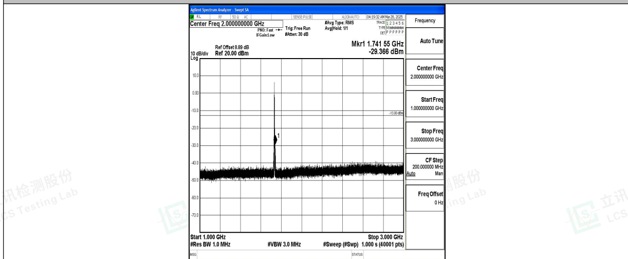
Band4_3MHz_16QAM_20175_1RB#0_1000~3000_1000~3000
