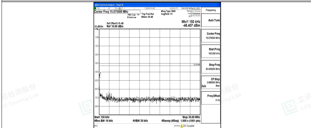
Band4_3MHz_QPSK_20385_1RB#0_0.15~30_0.15~30
