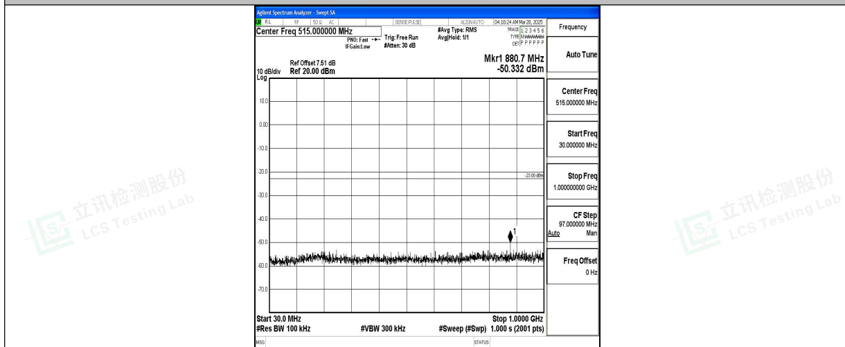
Band4_3MHz_16QAM_19965_1RB#0_30~1000_30~1000
