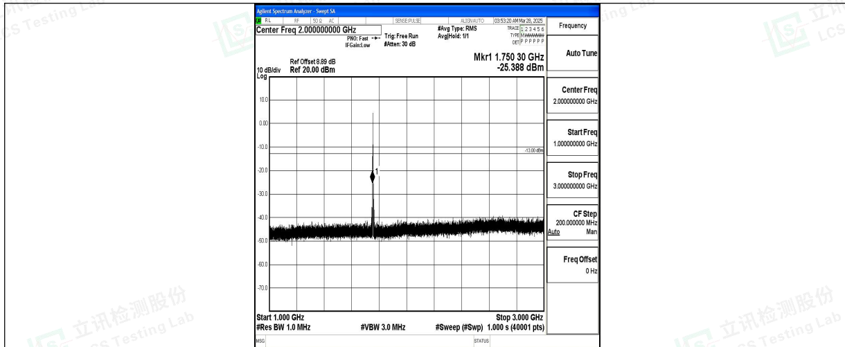
Band4_1.4MHz_QPSK_20393_1RB#0_1000~3000_1000~3000
