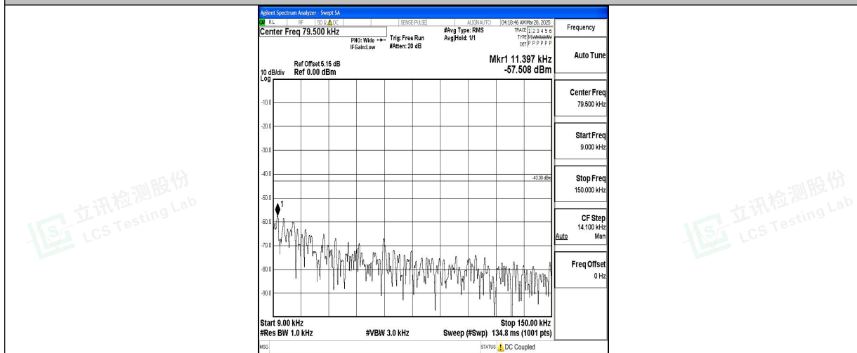
Band4_3MHz_QPSK_20175_1RB#0_0.009~0.15_0.009~0.15
