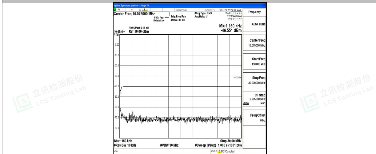
Band4_3MHz_QPSK_19965_1RB#0_0.15~30_0.15~30
