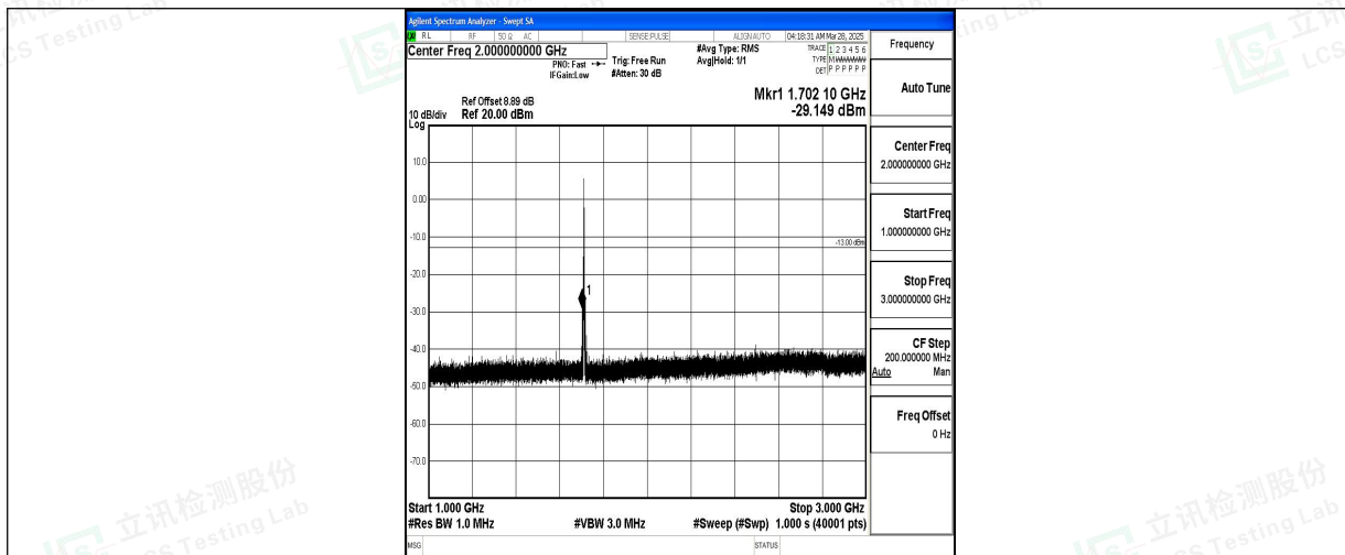
Band4_3MHz_16QAM_19965_1RB#0_1000~3000_1000~3000
