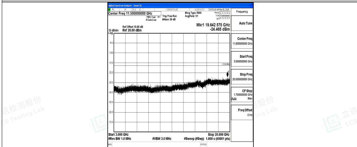
Band4_1.4MHz_QPSK_20393_1RB#0_3000~20000_3000~20000
