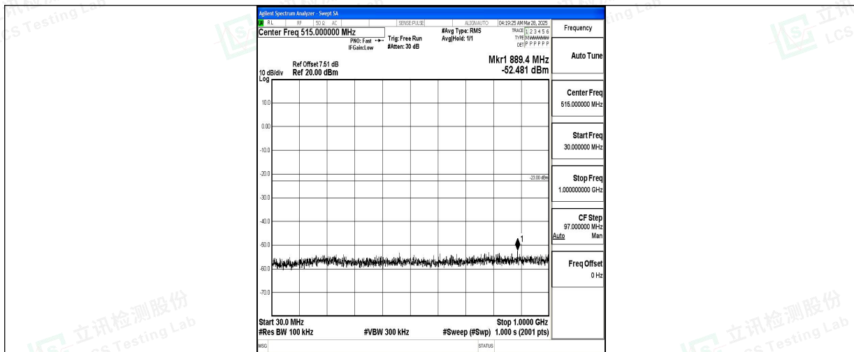
Band4_3MHz_16QAM_20175_1RB#0_30~1000_30~1000
