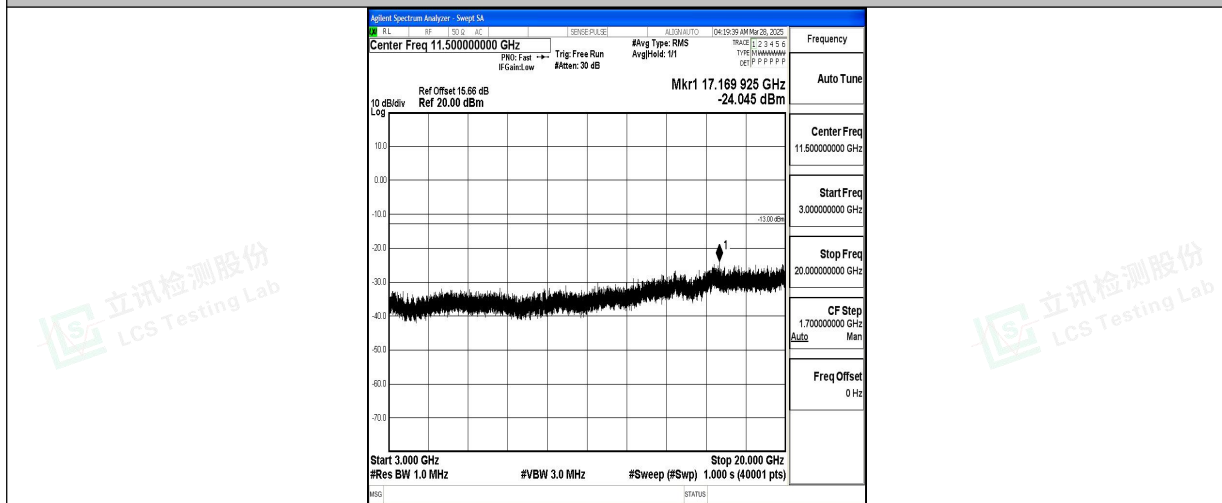
Band4_3MHz_16QAM_20175_1RB#0_3000~20000_3000~20000
