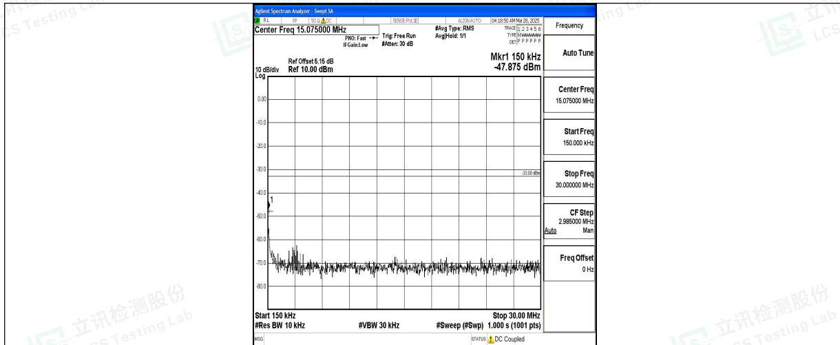
Band4_3MHz_QPSK_20175_1RB#0_0.15~30_0.15~30
