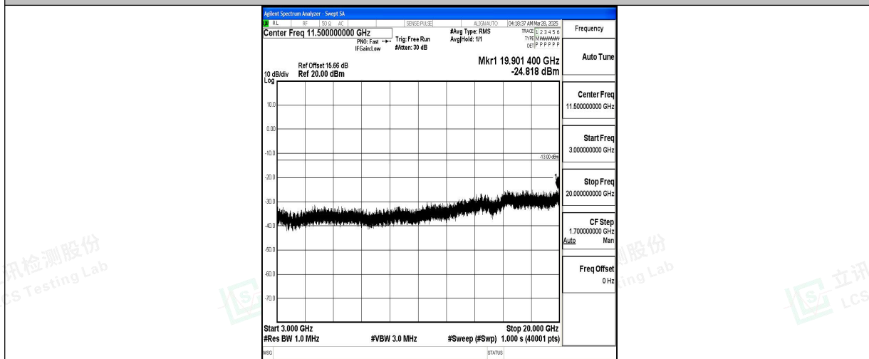
Band4_3MHz_16QAM_19965_1RB#0_3000~20000_3000~20000
