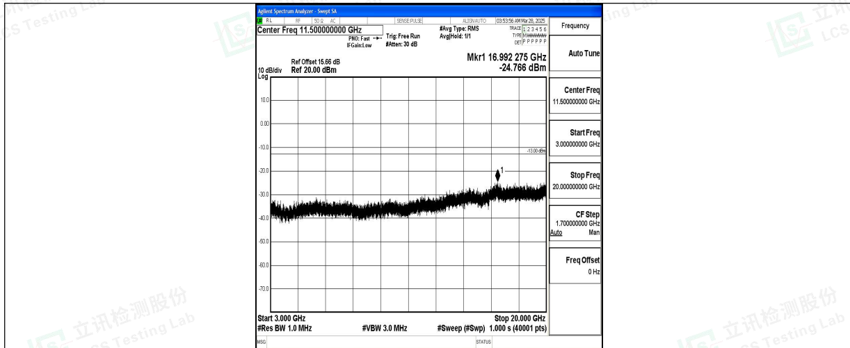
Band4_1.4MHz_16QAM_20393_1RB#0_3000~20000_3000~20000
