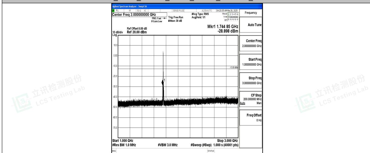
Band4_3MHz_16QAM_20385_1RB#0_1000~3000_1000~3000
