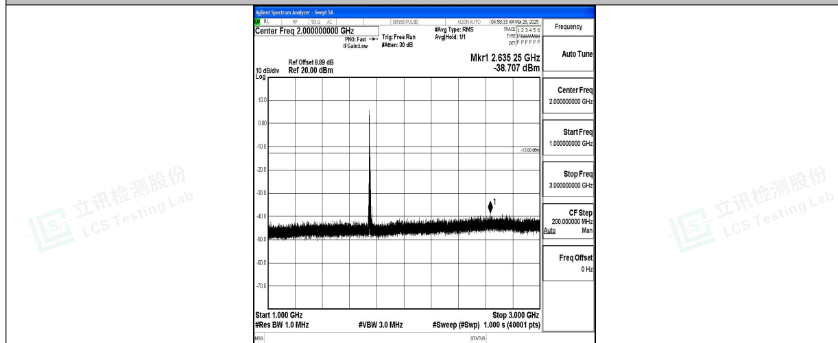
Band4_10MHz_16QAM_20350_1RB#0_1000~3000_1000~3000
