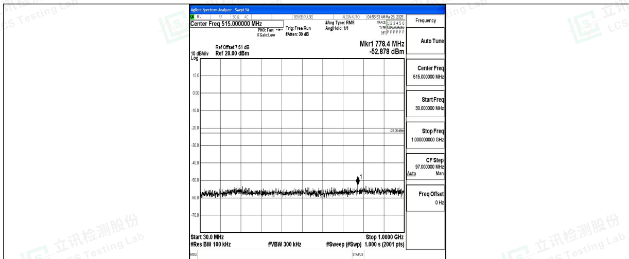
Band4_10MHz_QPSK_20000_1RB#0_30~1000_30~1000
