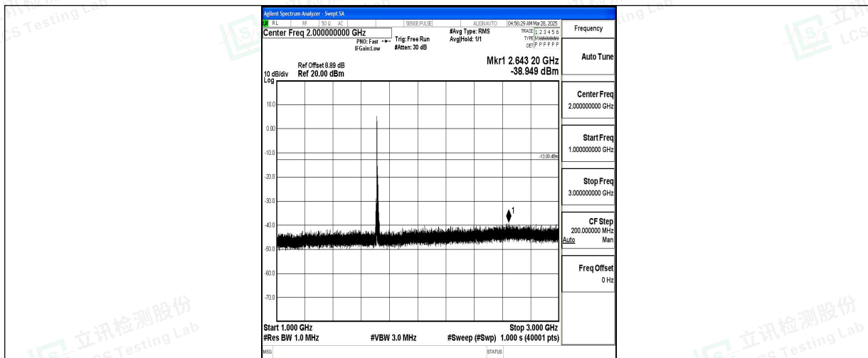
Band4_10MHz_16QAM_20000_1RB#0_1000~3000_1000~3000
