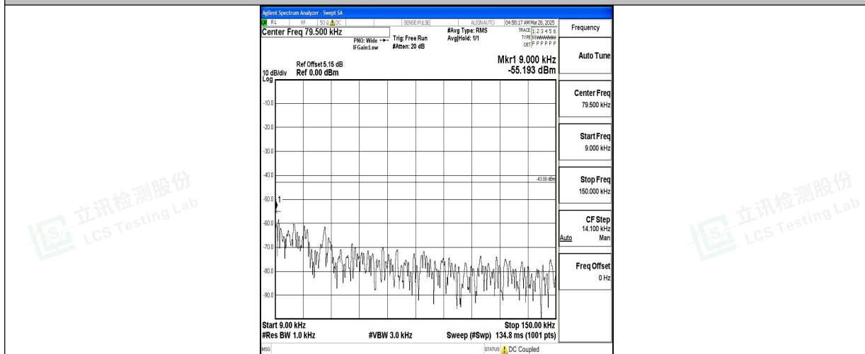
Band4_10MHz_16QAM_20350_1RB#0_0.009~0.15_0.009~0.15
