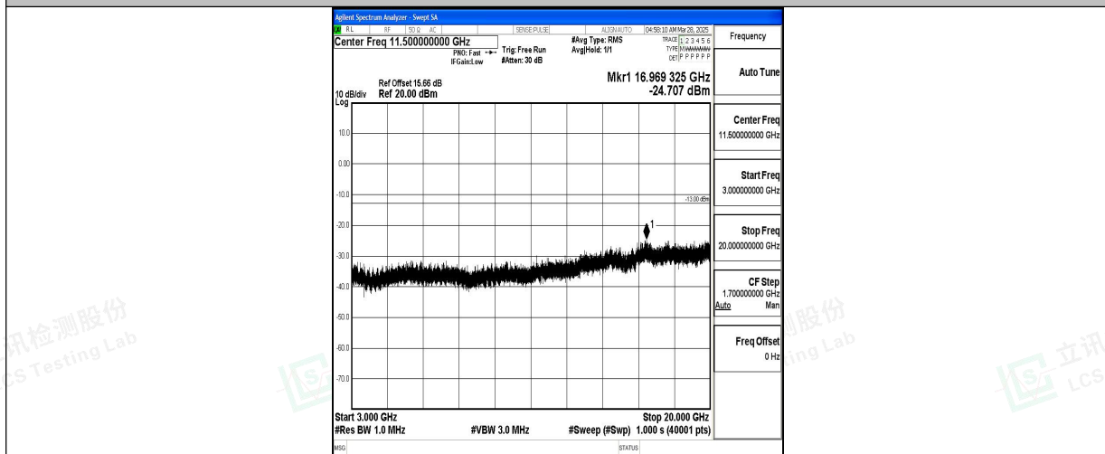
Band4_10MHz_QPSK_20350_1RB#0_3000~20000_3000~20000
