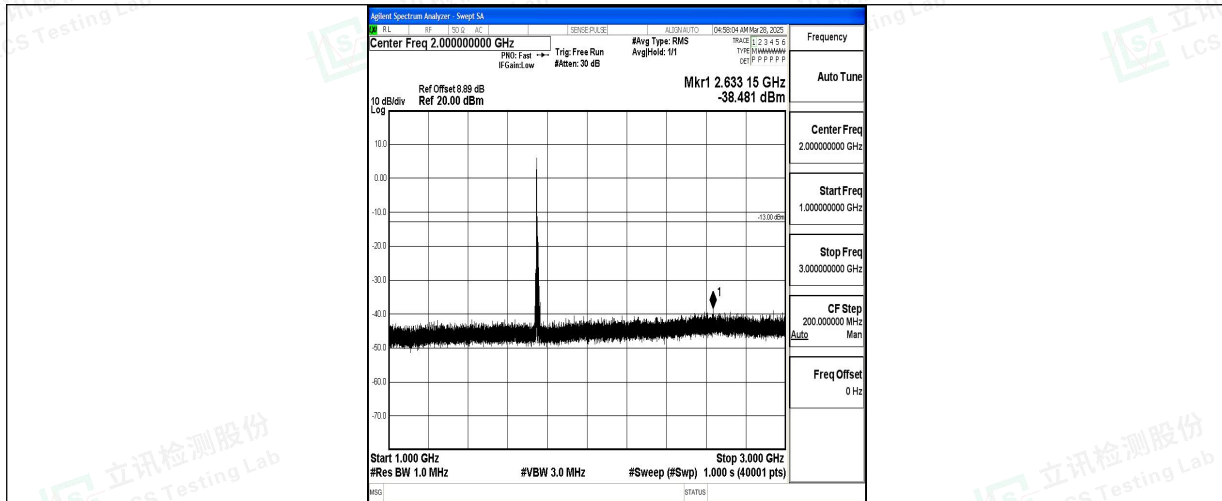
Band4_10MHz_QPSK_20350_1RB#0_1000~3000_1000~3000
