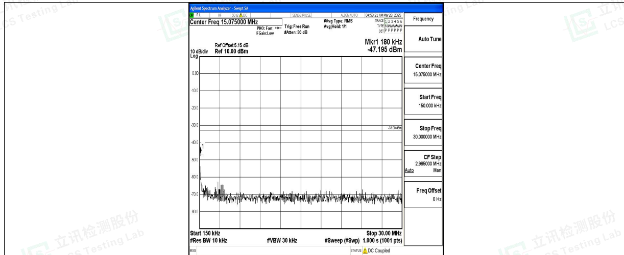
Band4_10MHz_16QAM_20350_1RB#0_0.15~30_0.15~30
