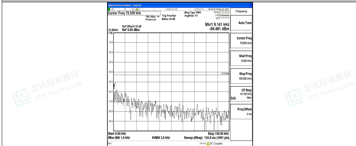
Band4_10MHz_QPSK_20175_1RB#0_0.009~0.15_0.009~0.15
