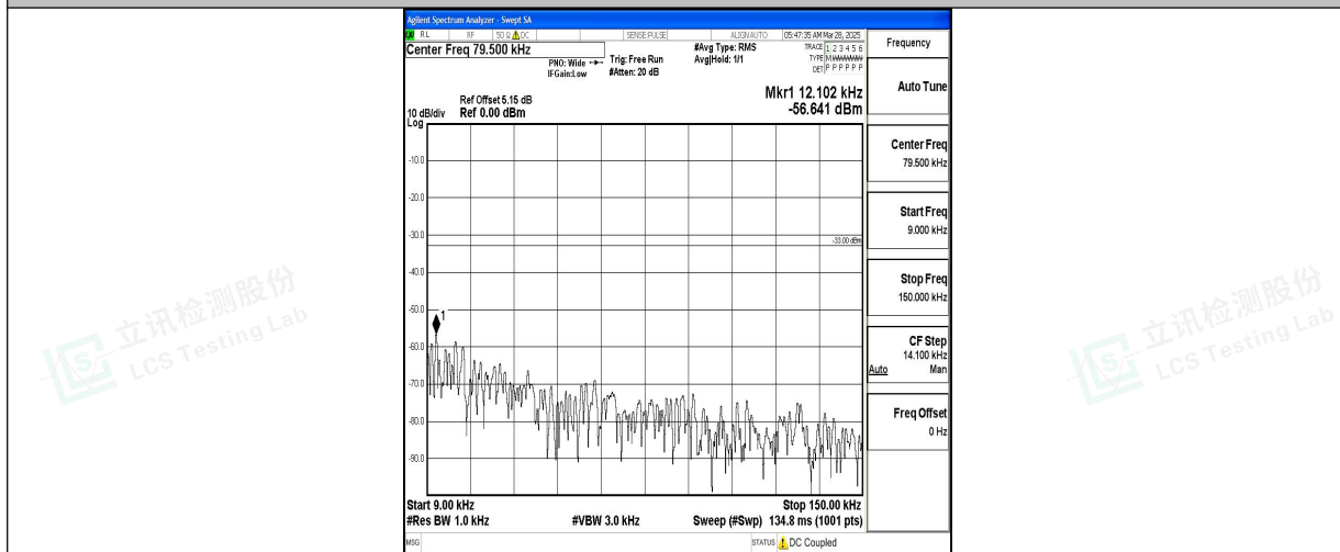
Band5_1.4MHz_QPSK_20643_1RB#0_0.009~0.15_0.009~0.15
