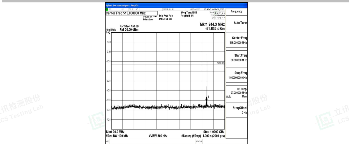
Band5_1.4MHz_QPSK_20643_1RB#0_30~1000_30~1000
