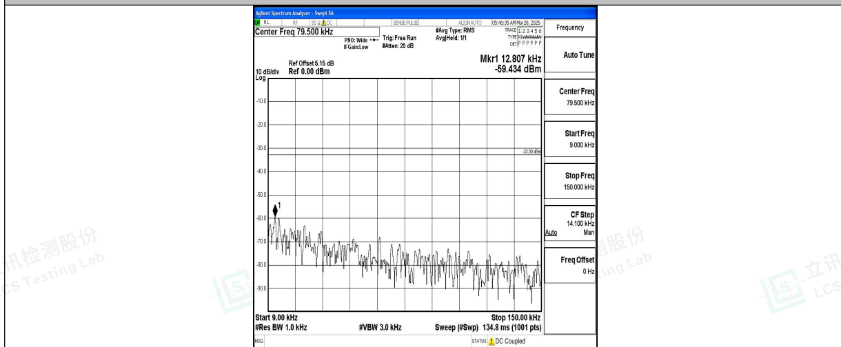
Band5_1.4MHz_QPSK_20525_1RB#0_0.009~0.15_0.009~0.15
