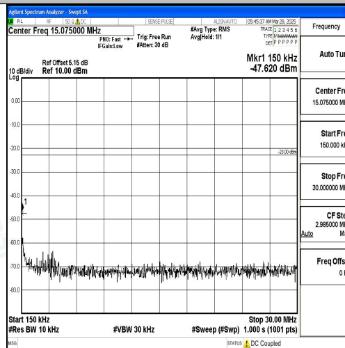
Band5_1.4MHz_QPSK_20407_1RB#0_0.15~30_0.15~30
