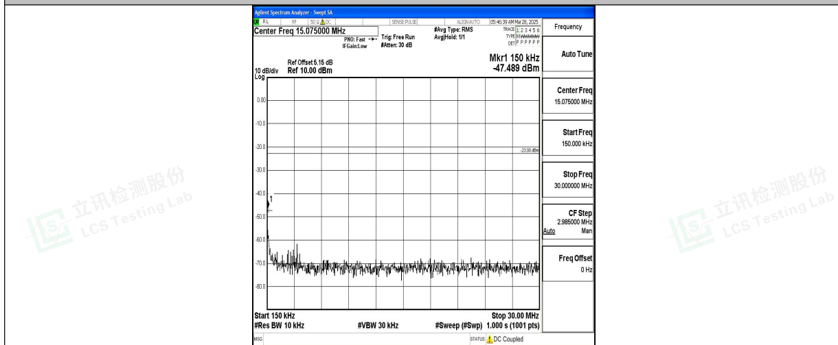
Band5_1.4MHz_QPSK_20525_1RB#0_0.15~30_0.15~30
