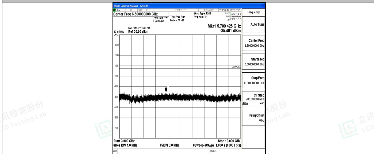
Band5_1.4MHz_16QAM_20525_1RB#0_3000~10000_3000~10000
