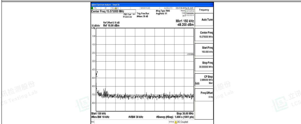
Band5_1.4MHz_16QAM_20525_1RB#0_0.15~30_0.15~30
