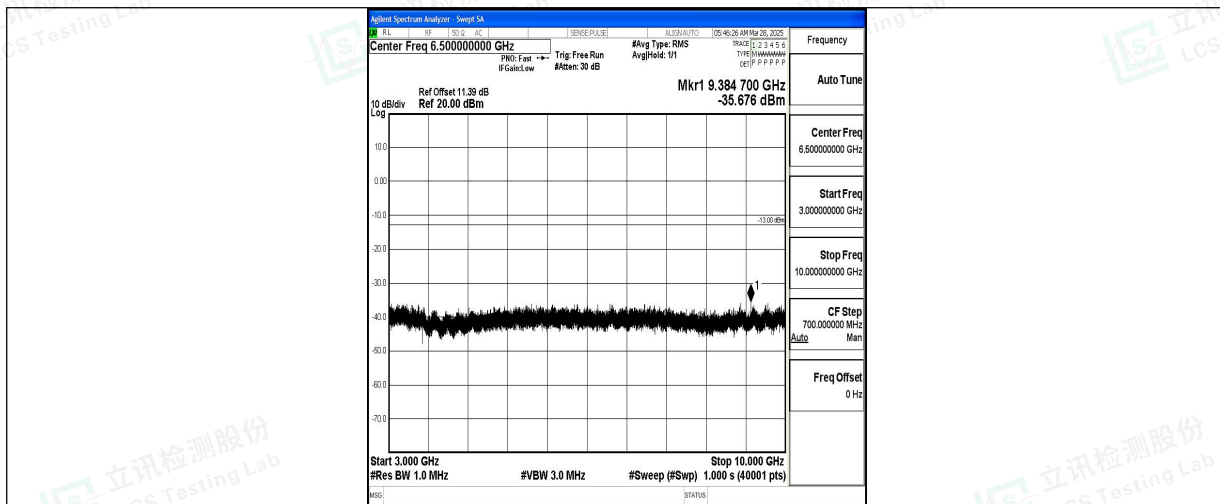
Band5_1.4MHz_16QAM_20407_1RB#0_3000~10000_3000~10000
