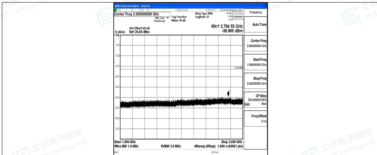
Band5_1.4MHz_QPSK_20407_1RB#0_1000~3000_1000~3000
