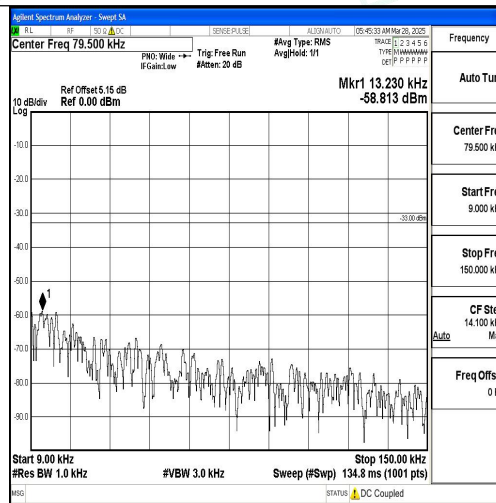
Band5_1.4MHz_QPSK_20407_1RB#0_0.009~0.15_0.009~0.15
