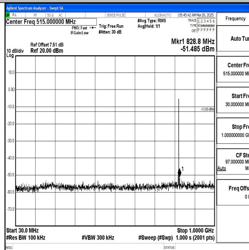
Band5_1.4MHz_QPSK_20407_1RB#0_30~1000_30~1000
