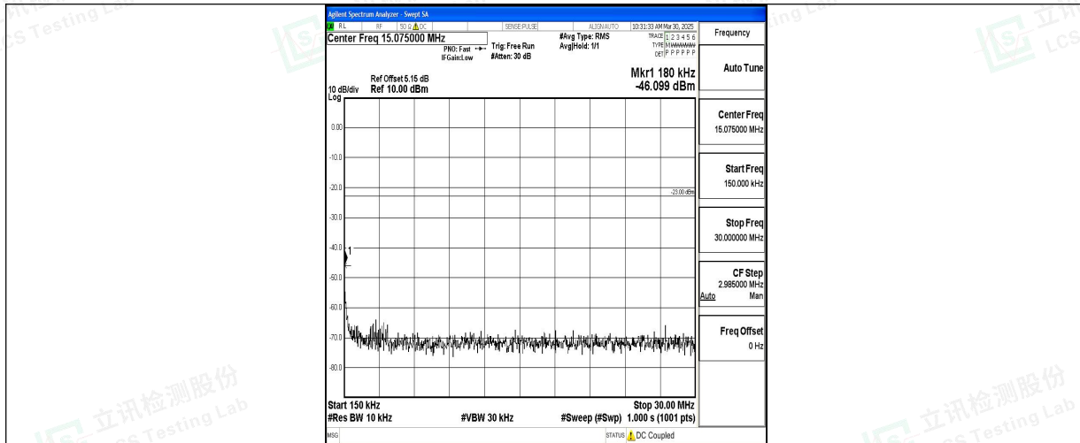
Band5_3MHz_16QAM_20415_1RB#0_0.15~30_0.15~30
