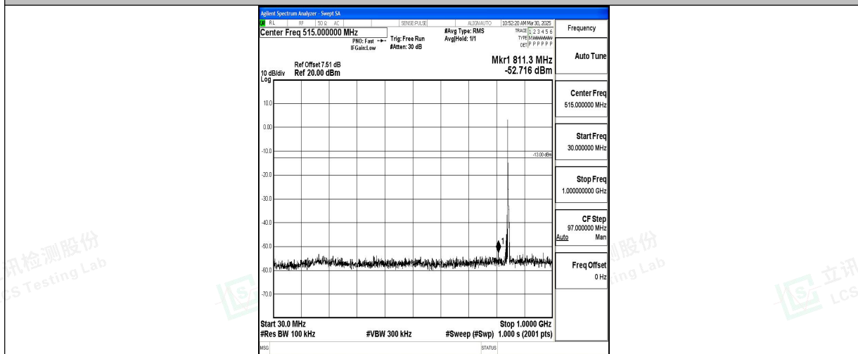
Band5_5MHz_QPSK_20625_1RB#0_30~1000_30~1000
