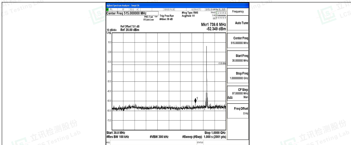
Band5_5MHz_QPSK_20525_1RB#0_30~1000_30~1000
