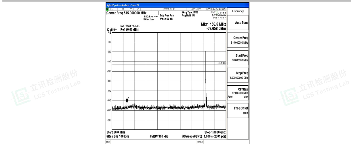
Band5_5MHz_QPSK_20425_1RB#0_30~1000_30~1000
