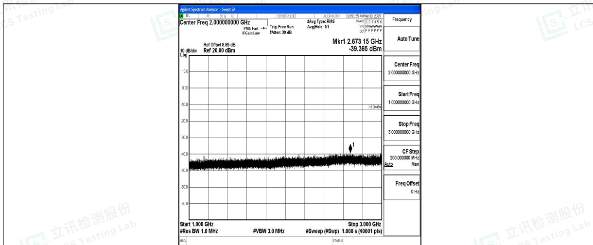
Band5_5MHz_16QAM_20525_1RB#0_1000~3000_1000~3000
