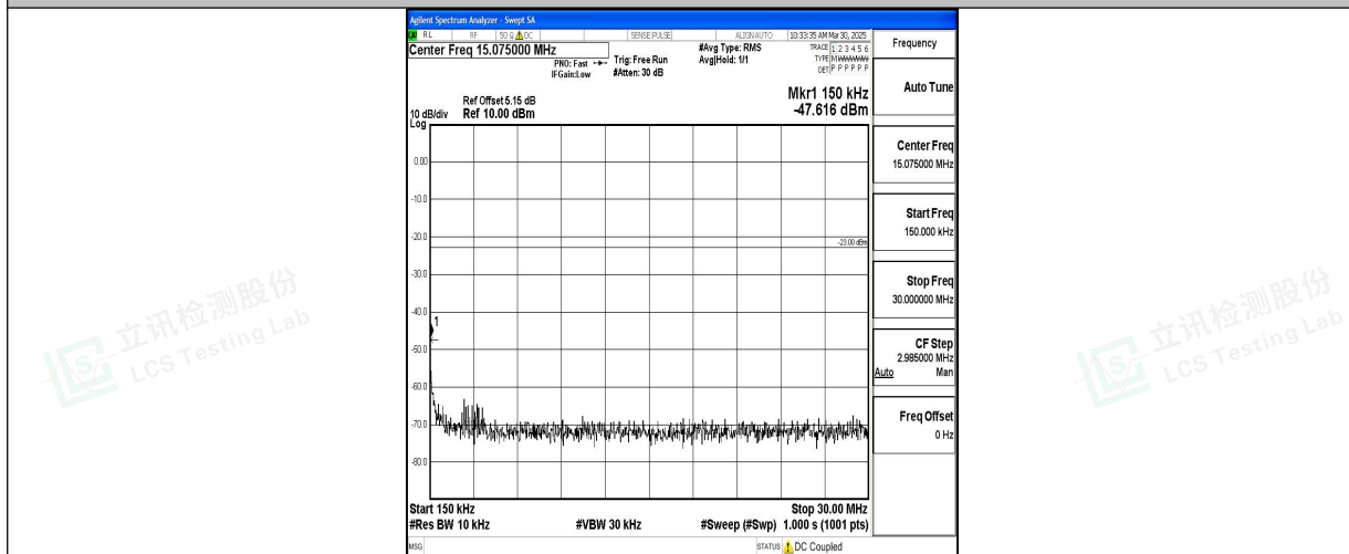
Band5_3MHz_16QAM_20635_1RB#0_0.15~30_0.15~30
