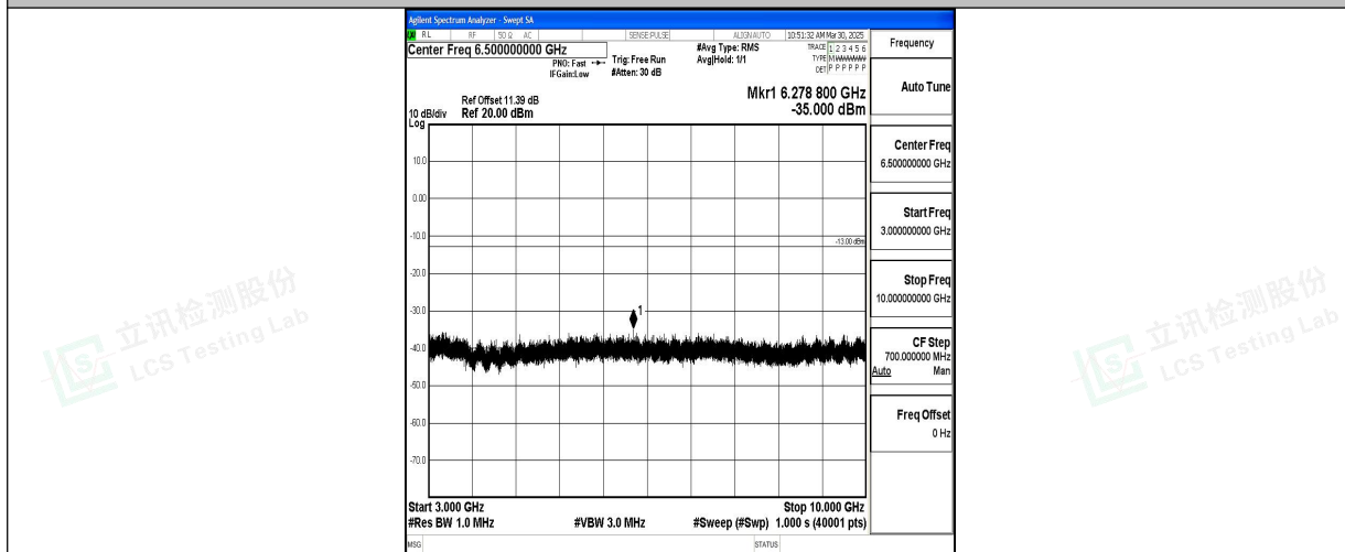
Band5_5MHz_QPSK_20525_1RB#0_3000~10000_3000~10000
