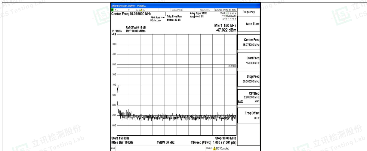
Band5_5MHz_QPSK_20625_1RB#0_0.15~30_0.15~30
