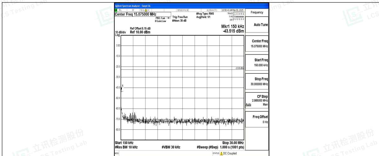
Band5_5MHz_16QAM_20425_1RB#0_0.15~30_0.15~30
