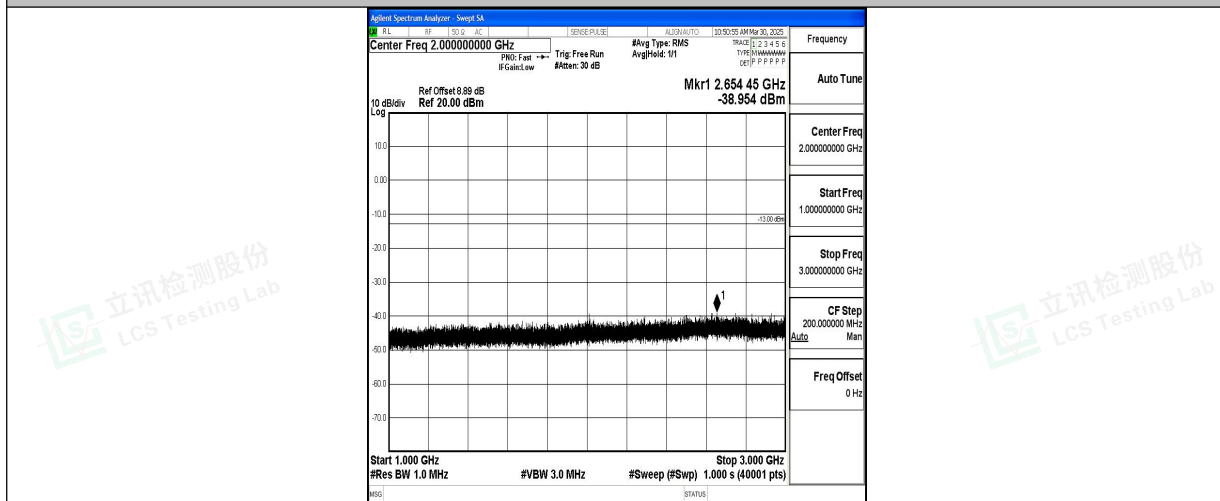
Band5_5MHz_16QAM_20425_1RB#0_1000~3000_1000~3000
