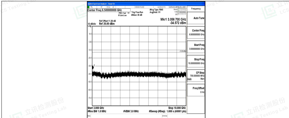
Band5_5MHz_16QAM_20425_1RB#0_3000~10000_3000~10000
