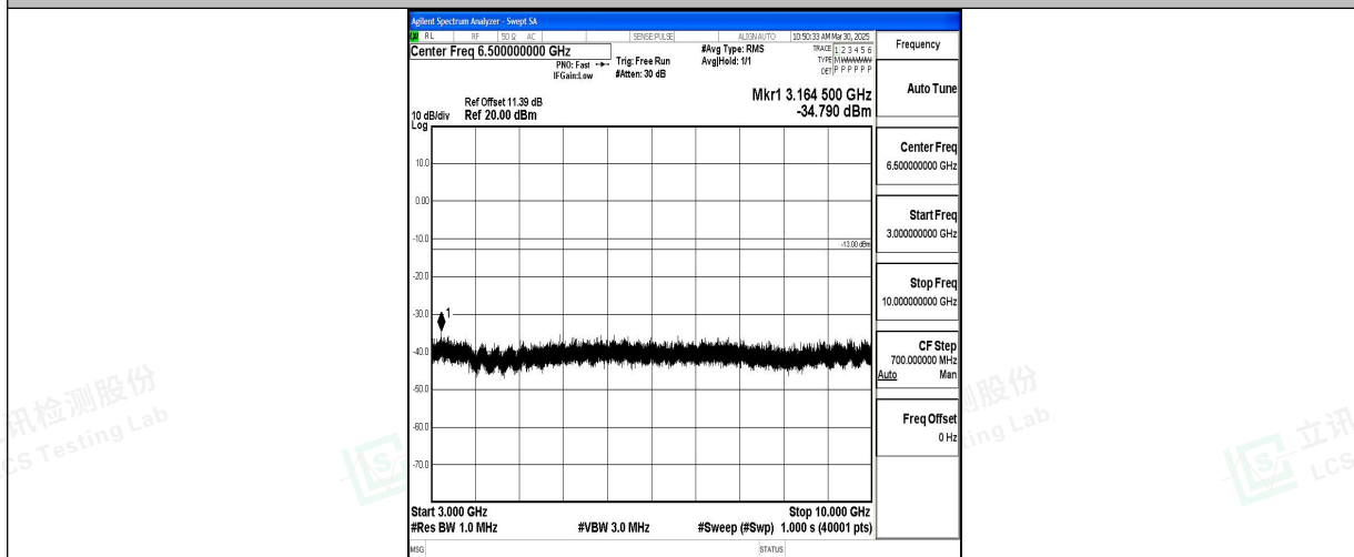
Band5_5MHz_QPSK_20425_1RB#0_3000~10000_3000~10000
