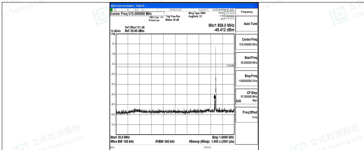
Band5_3MHz_16QAM_20635_1RB#0_30~1000_30~1000
