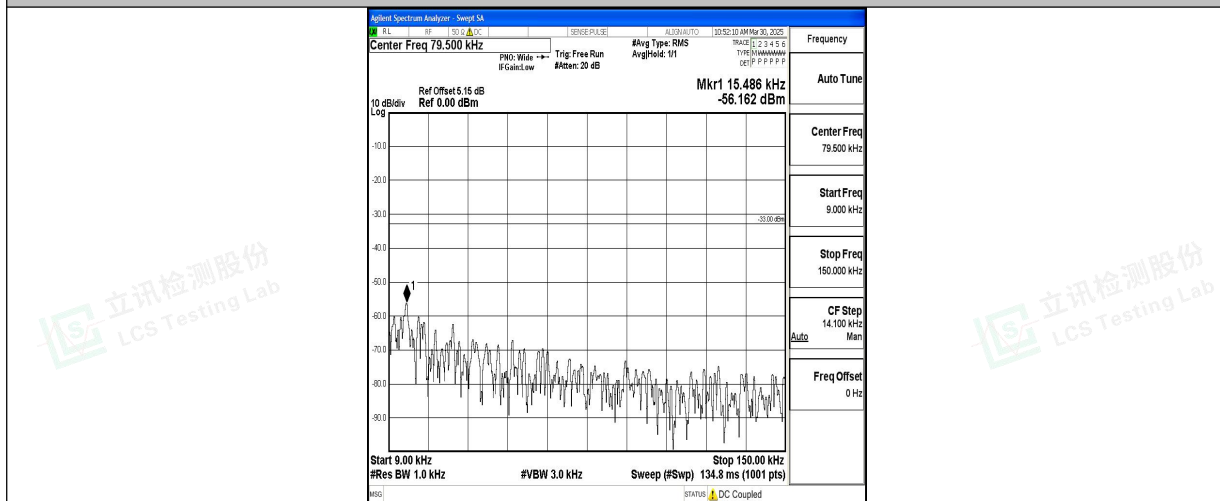
Band5_5MHz_QPSK_20625_1RB#0_0.009~0.15_0.009~0.15
