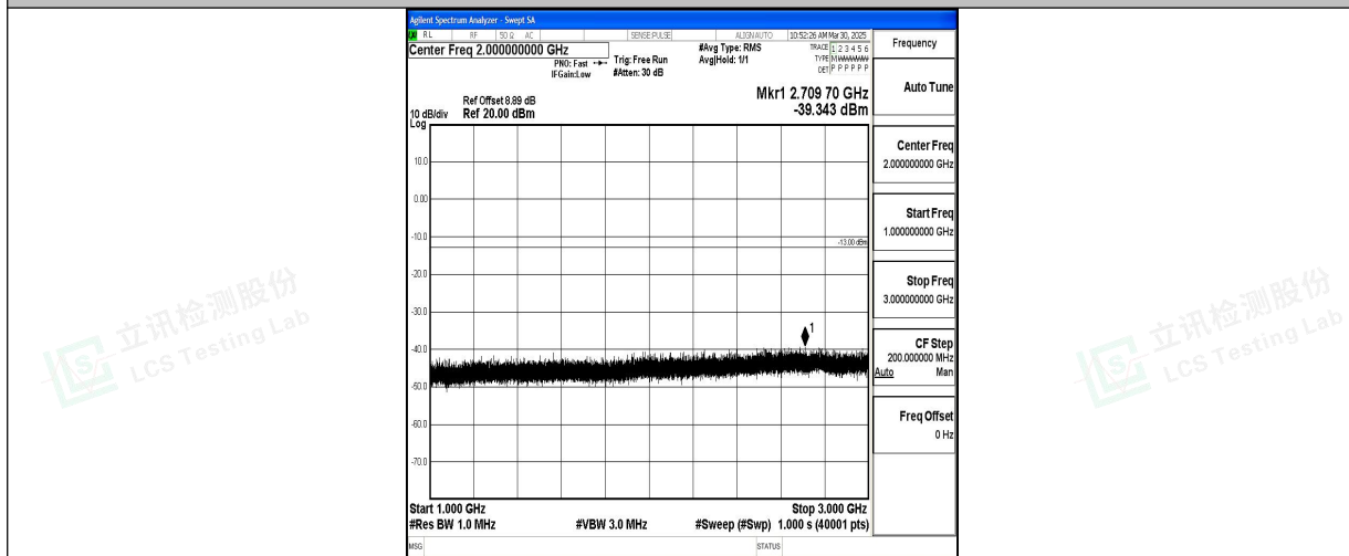
Band5_5MHz_QPSK_20625_1RB#0_1000~3000_1000~3000
