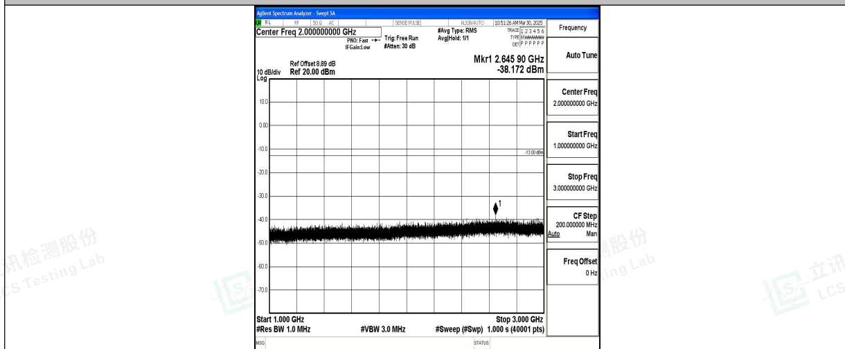
Band5_5MHz_QPSK_20525_1RB#0_1000~3000_1000~3000
