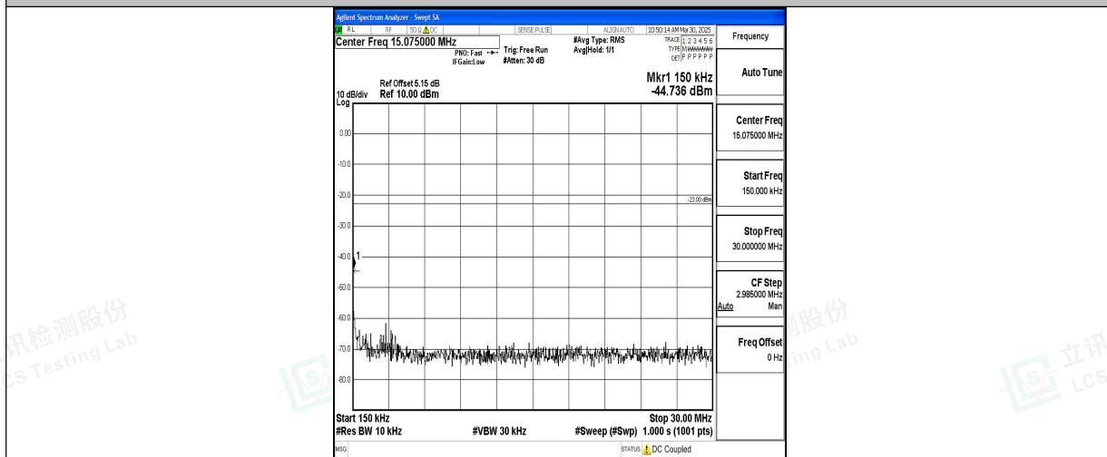
Band5_5MHz_QPSK_20425_1RB#0_0.15~30_0.15~30
