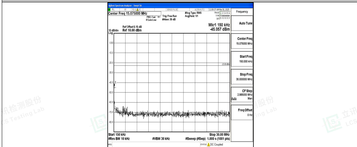
Band5_10MHz_16QAM_20525_1RB#0_0.15~30_0.15~30
