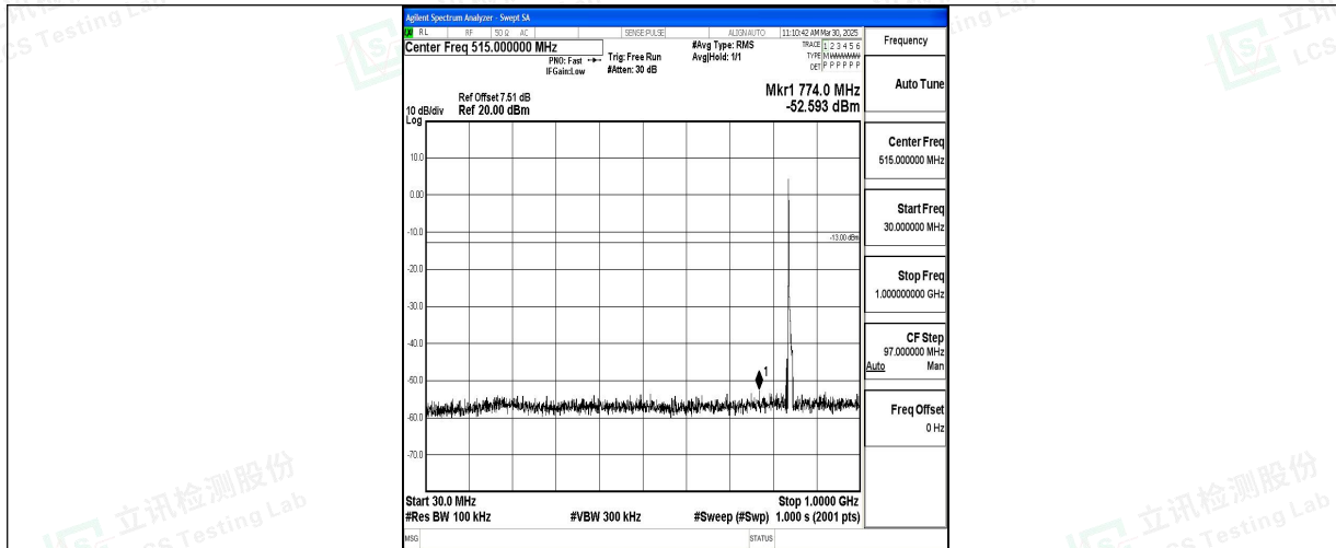
Band5_10MHz_16QAM_20600_1RB#0_30~1000_30~1000
