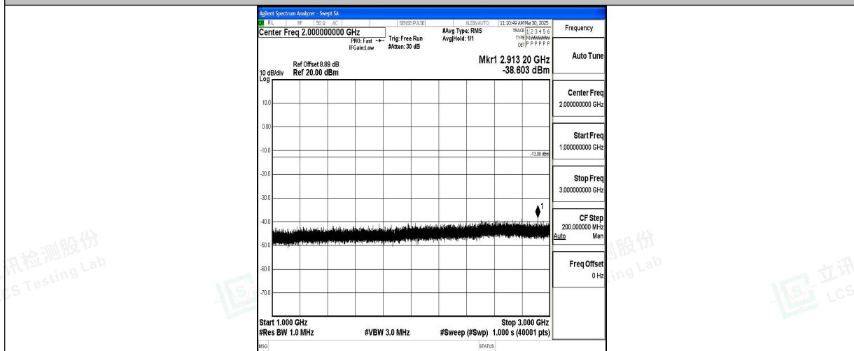
Band5_10MHz_16QAM_20600_1RB#0_1000~3000_1000~3000
