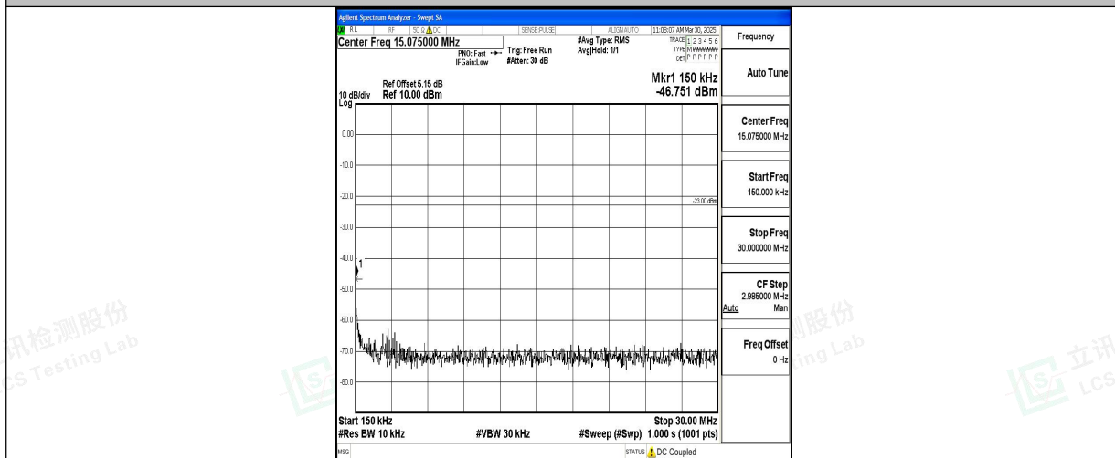
Band5_10MHz_QPSK_20450_1RB#0_0.15~30_0.15~30
