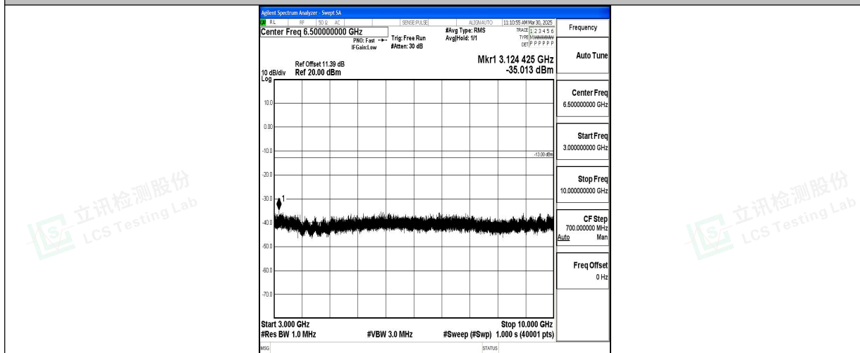
Band5_10MHz_16QAM_20600_1RB#0_3000~10000_3000~10000
