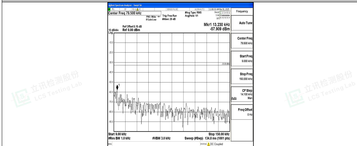
Band5_10MHz_16QAM_20450_1RB#0_0.009~0.15_0.009~0.15
