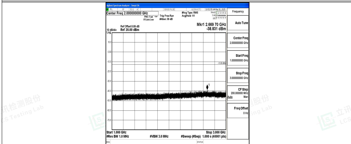
Band5_5MHz_16QAM_20625_1RB#0_1000~3000_1000~3000
