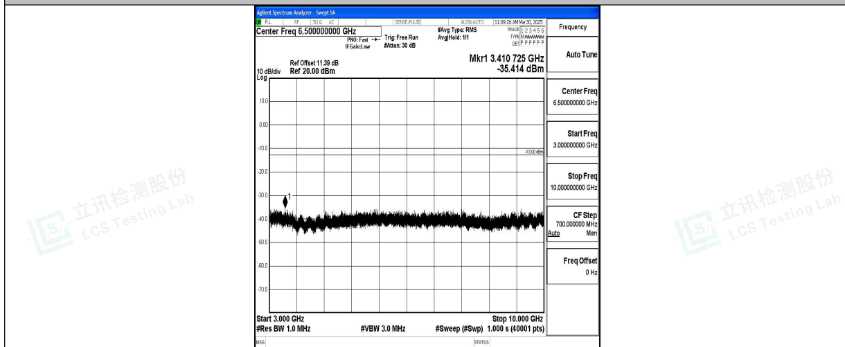
Band5_10MHz_QPSK_20525_1RB#0_3000~10000_3000~10000
