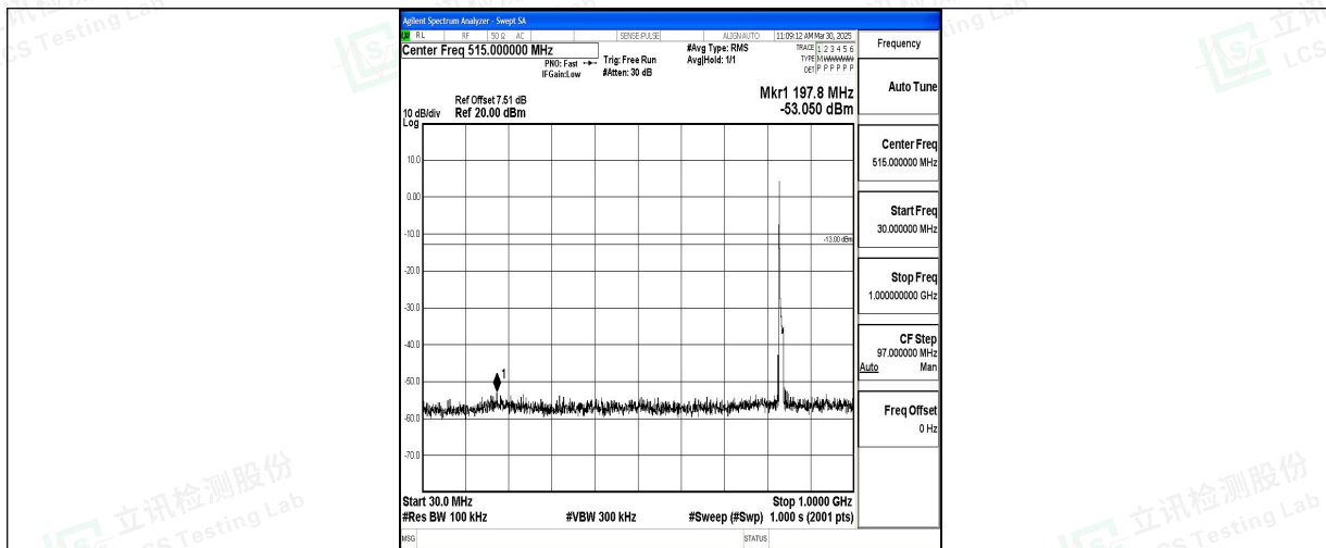
Band5_10MHz_QPSK_20525_1RB#0_30~1000_30~1000
