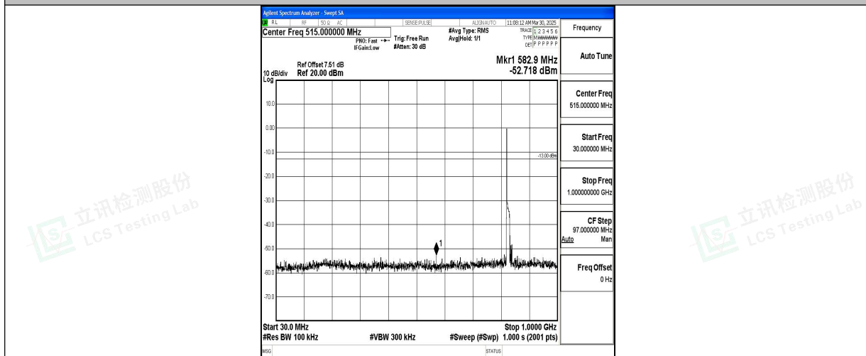
Band5_10MHz_QPSK_20450_1RB#0_30~1000_30~1000
