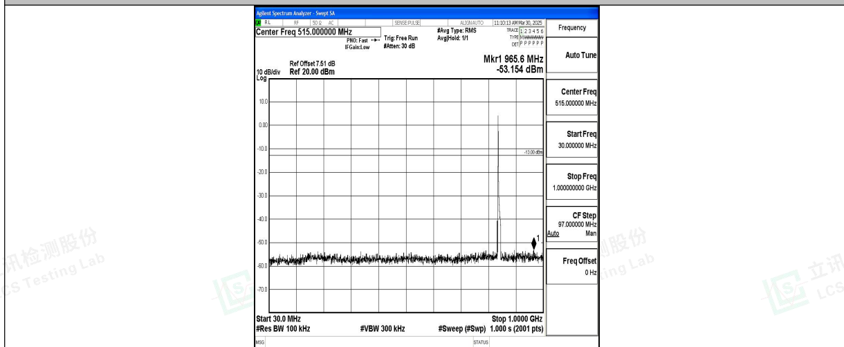
Band5_10MHz_QPSK_20600_1RB#0_30~1000_30~1000
