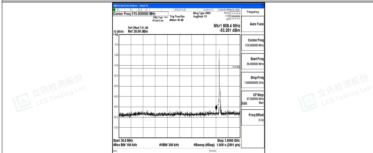
Band5_10MHz_16QAM_20525_1RB#0_30~1000_30~1000
