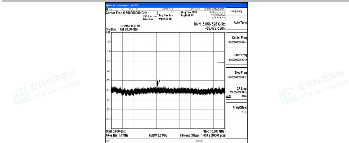
Band5_5MHz_16QAM_20625_1RB#0_3000~10000_3000~10000
