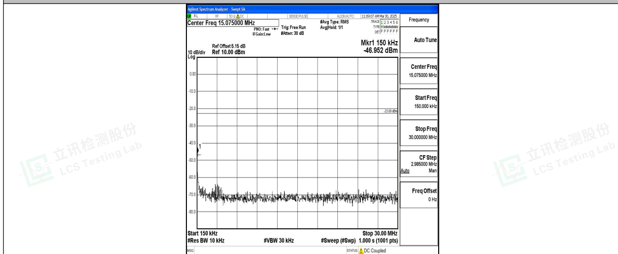
Band5_10MHz_QPSK_20525_1RB#0_0.15~30_0.15~30
