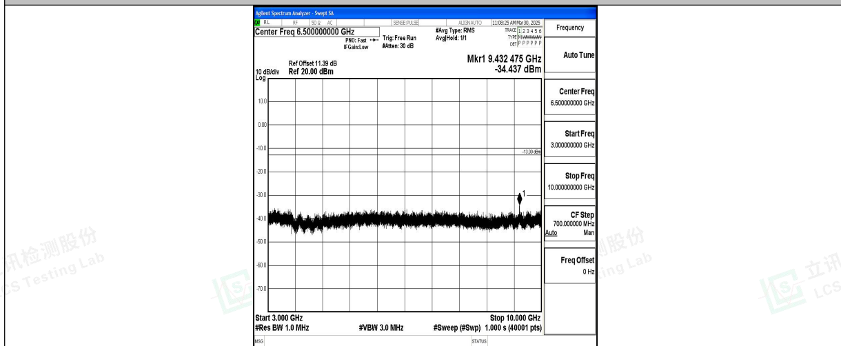
Band5_10MHz_QPSK_20450_1RB#0_3000~10000_3000~10000
