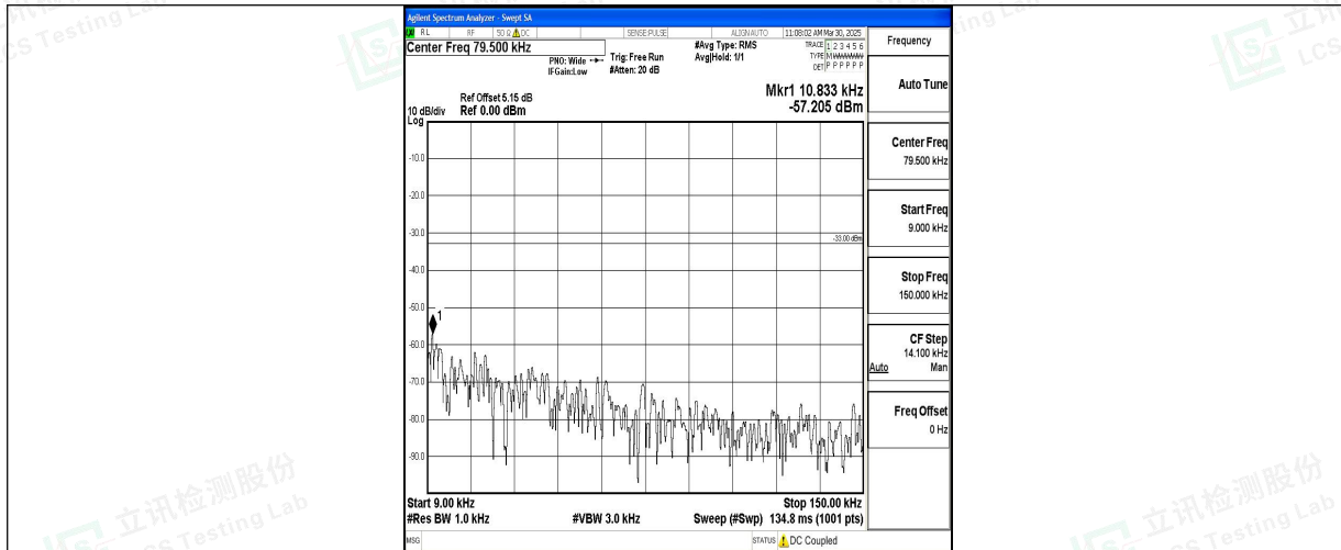
Band5_10MHz_QPSK_20450_1RB#0_0.009~0.15_0.009~0.15
