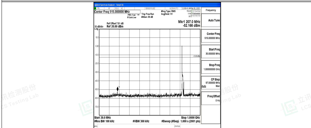
Band5_10MHz_16QAM_20450_1RB#0_30~1000_30~1000
