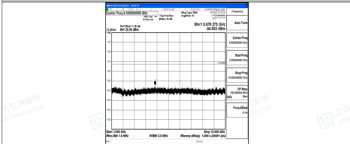
Band5_10MHz_16QAM_20525_1RB#0_3000~10000_3000~10000
