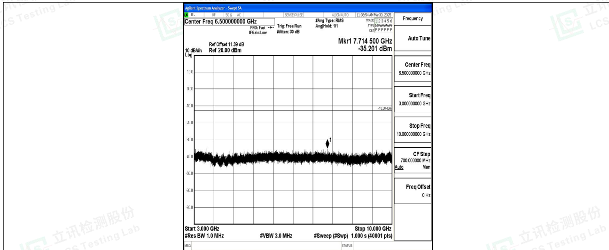
Band5_10MHz_16QAM_20450_1RB#0_3000~10000_3000~10000
