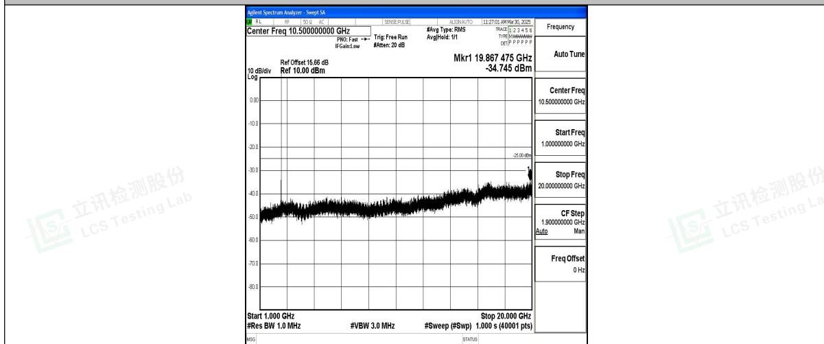
Band7_5MHz_16QAM_20775_1RB#0_1000~20000_1000~20000
