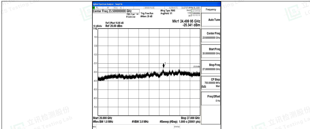
Band7_5MHz_16QAM_20775_1RB#0_20000~27000_20000~27000
