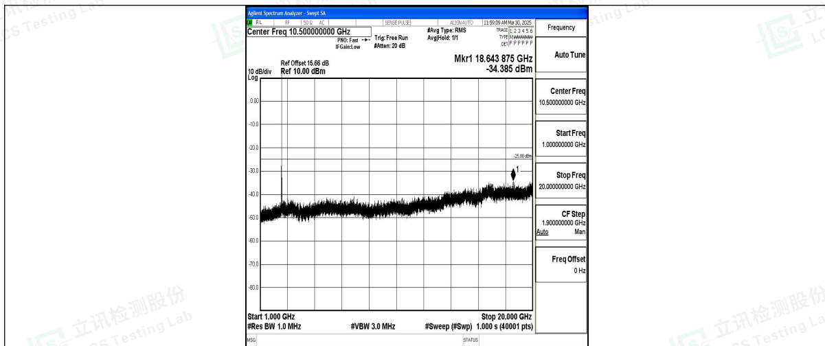
Band7_15MHz_QPSK_20825_1RB#0_1000~20000_1000~20000
