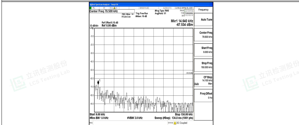
Band7_15MHz_16QAM_20825_1RB#0_0.009~0.15_0.009~0.15
