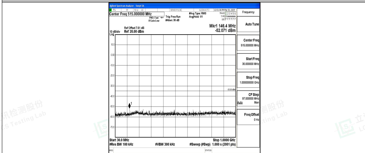
Band7_15MHz_QPSK_21375_1RB#0_30~1000_30~1000
