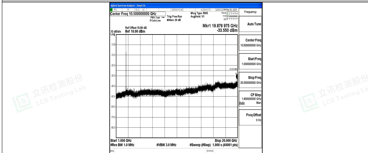
Band7_15MHz_QPSK_21375_1RB#0_1000~20000_1000~20000
