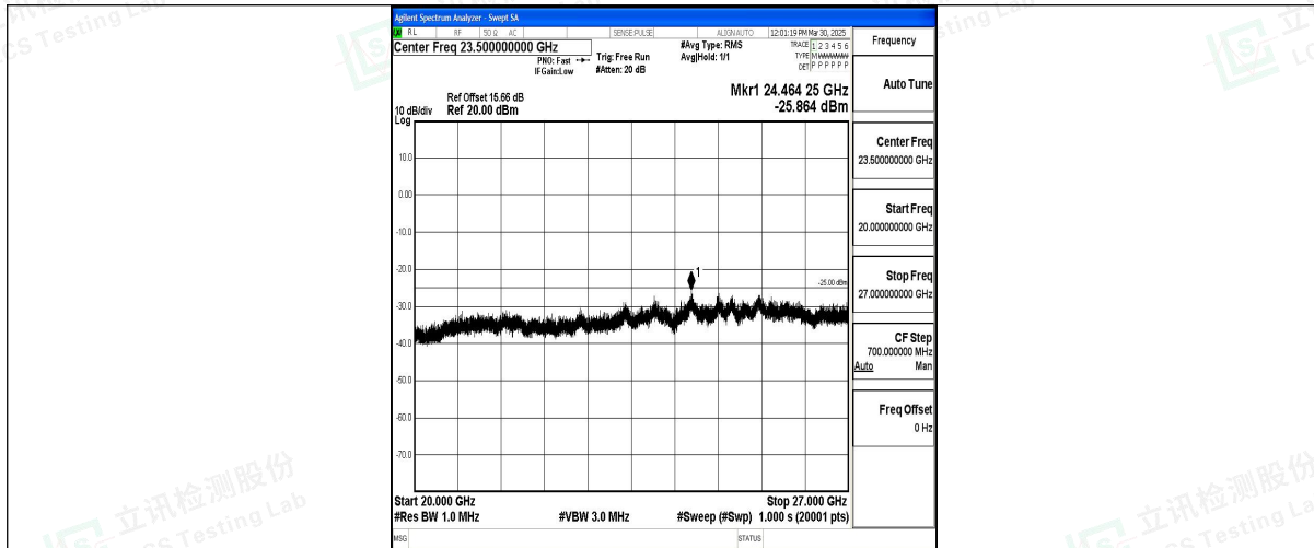
Band7_15MHz_QPSK_21375_1RB#0_20000~27000_20000~27000
