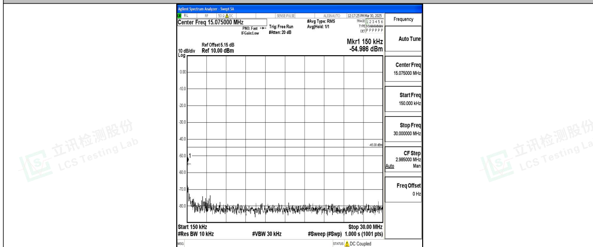
Band7_20MHz_16QAM_21350_1RB#0_0.15~30_0.15~30
