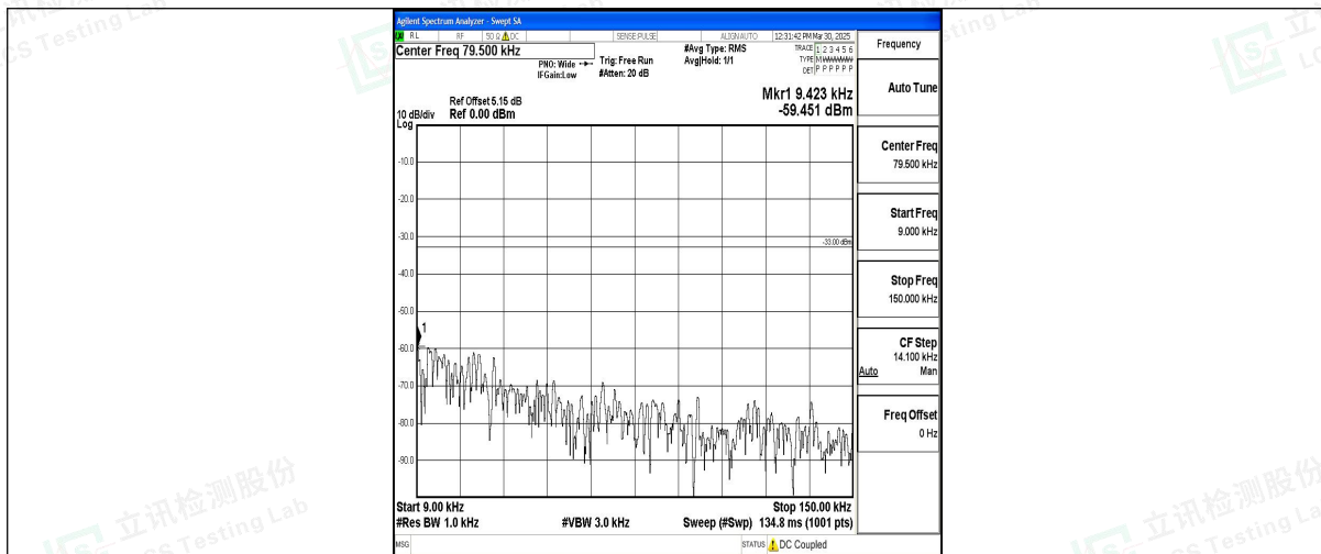
Band12_1.4MHz_16QAM_23095_1RB#0_0.009~0.15_0.009~0.15
