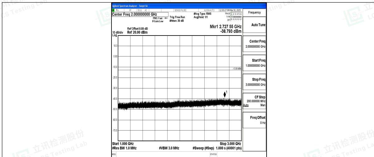
Band12_1.4MHz_QPSK_23017_1RB#0_1000~3000_1000~3000
