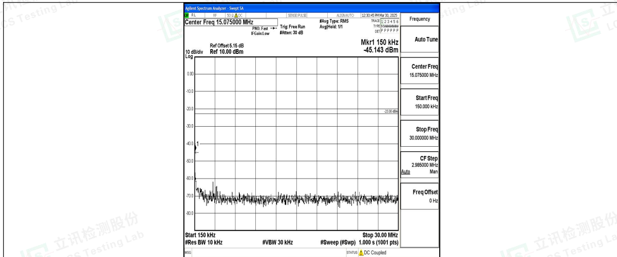
Band12_1.4MHz_16QAM_23017_1RB#0_0.15~30_0.15~30
