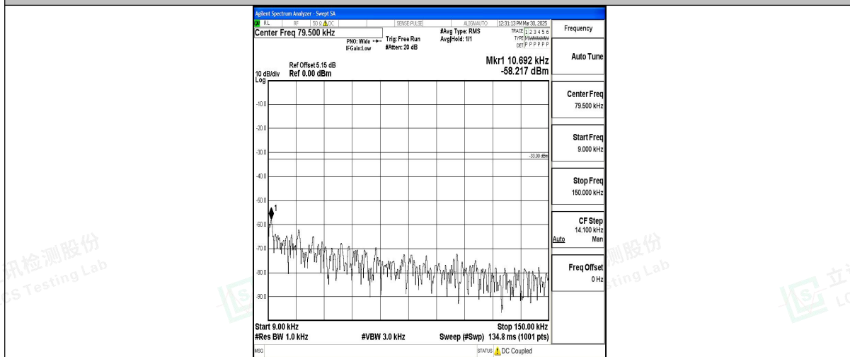
Band12_1.4MHz_QPSK_23095_1RB#0_0.009~0.15_0.009~0.15
