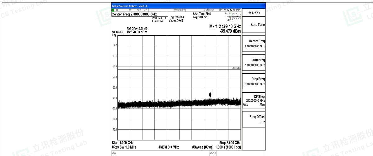
Band12_1.4MHz_16QAM_23095_1RB#0_1000~3000_1000~3000
