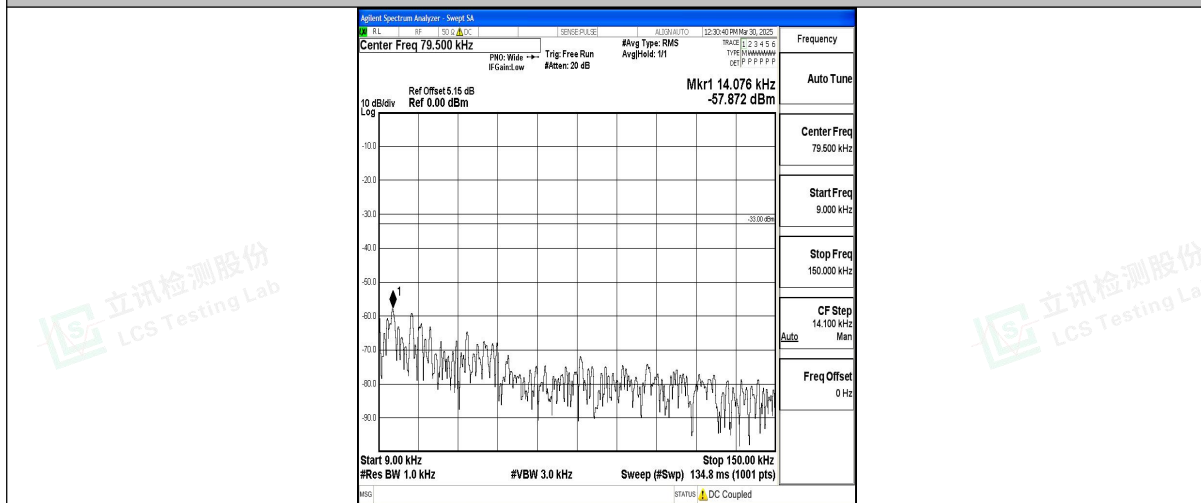
Band12_1.4MHz_16QAM_23017_1RB#0_0.009~0.15_0.009~0.15
