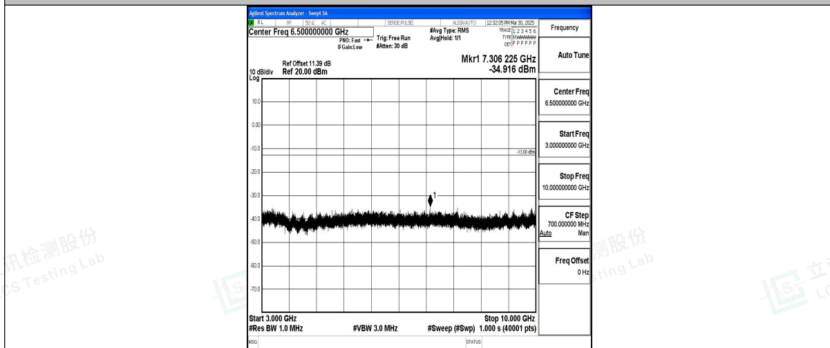
Band12_1.4MHz_16QAM_23095_1RB#0_3000~10000_3000~10000
