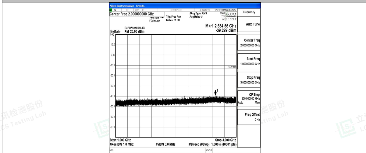
Band12_1.4MHz_QPSK_23095_1RB#0_1000~3000_1000~3000
