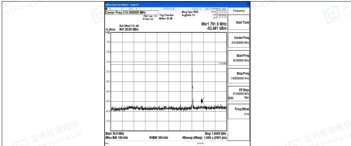
Band12_5MHz_16QAM_23155_1RB#0_30~1000_30~1000
