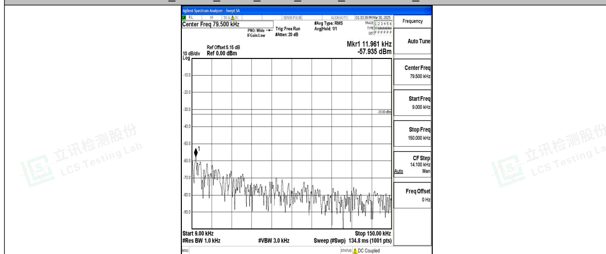
Band12_10MHz_16QAM_23060_1RB#0_0.009~0.15_0.009~0.15
