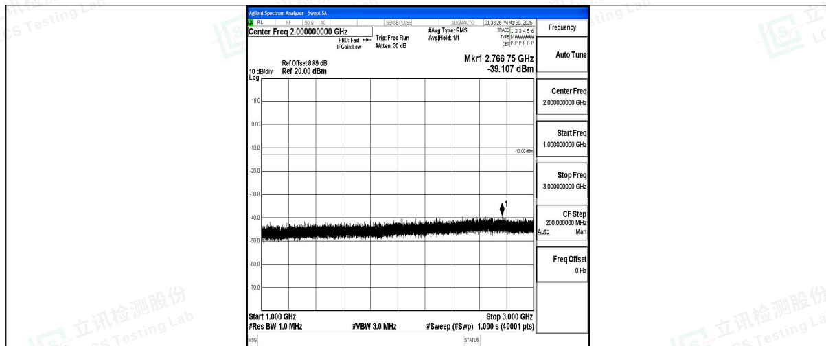
Band12_10MHz_QPSK_23060_1RB#0_1000~3000_1000~3000
