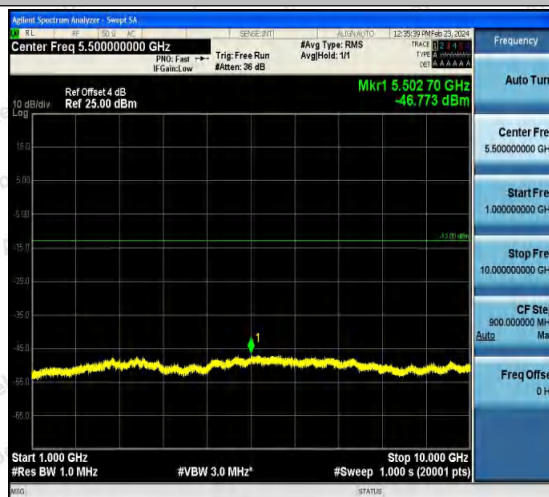
Band5-4233-4-1000~10000MHz-PASS
