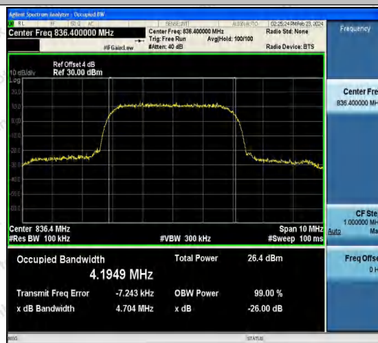
Band5-4182-1-PASS
