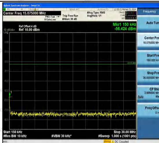
Band5-4233-4-0.15~30MHz-PASS
