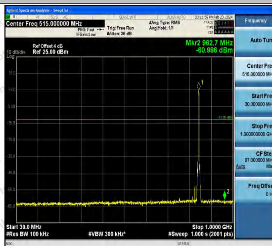
Band5-4233-5-30~1000MHz-PASS
