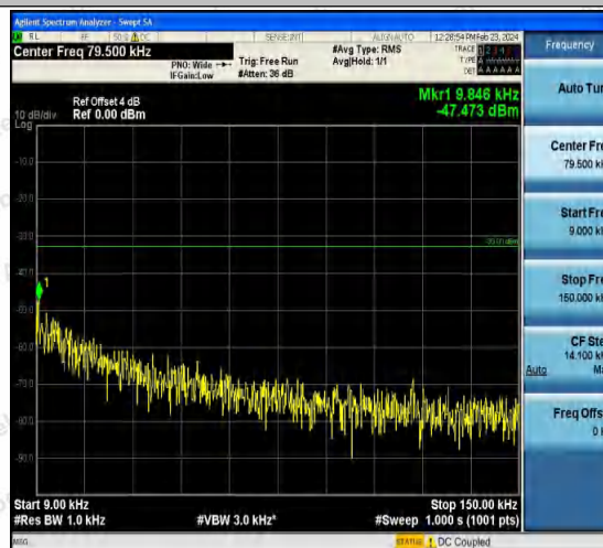
Band5-4233-1-0.009~0.15MHz-PASS
