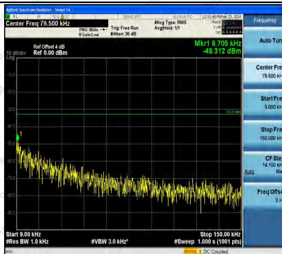
Band5-4132-3-0.009~0.15MHz-PASS
