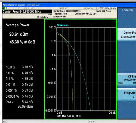
Band5-4233-3-PASS
