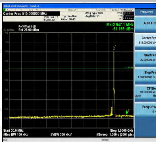
Band5-4233-4-30~1000MHz-PASS
