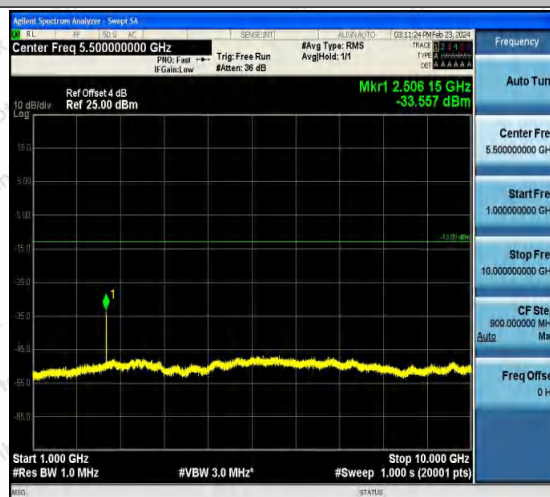
Band5-4182-5-1000~10000MHz-PASS
