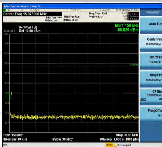
Band5-4132-3-0.15~30MHz-PASS
