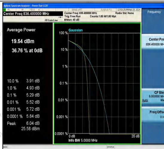
Band5-4182-2-PASS
