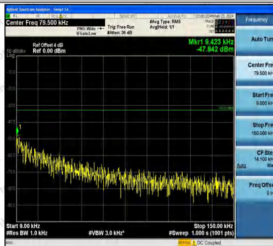
Band5-4182-2-0.009~0.15MHz-PASS
