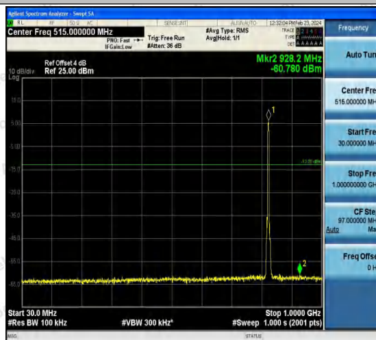
Band5-4132-3-30~1000MHz-PASS
