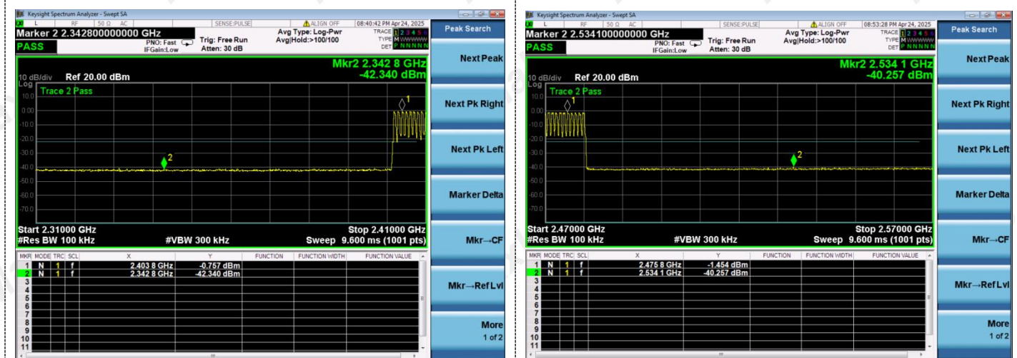
Left Band edge hopping on
