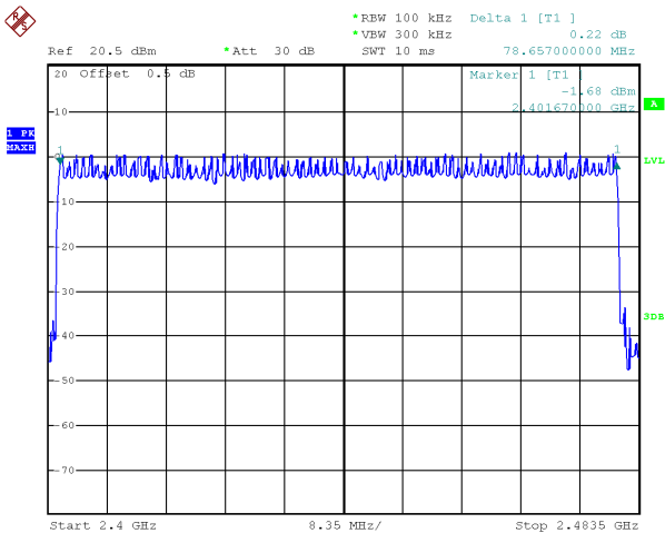
Modulation: 8DPSK
