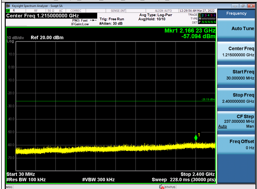
Test_Graph_LE1M_ANT1_2471_1Mbps_Lower Band Emissions
