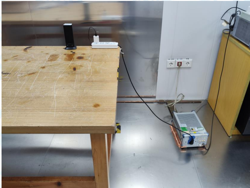
Photo of Setup for Conducted Emission
