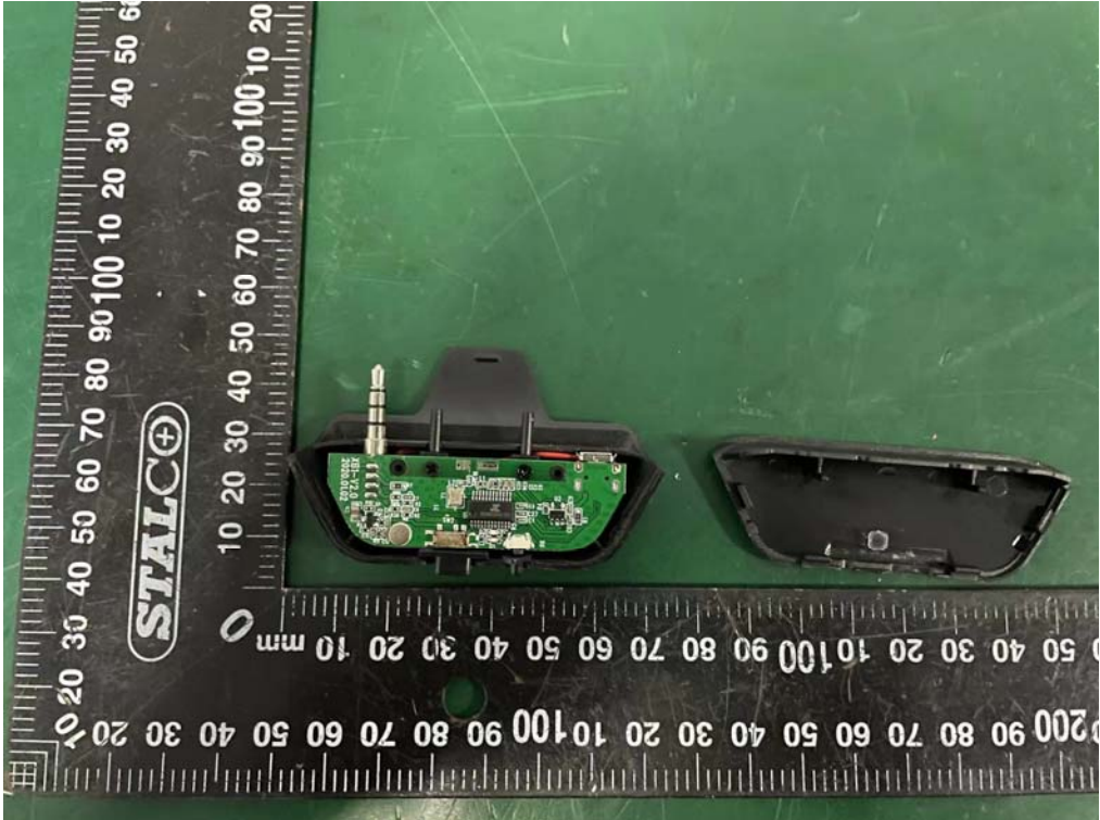
Internal Photos M/N: U002
