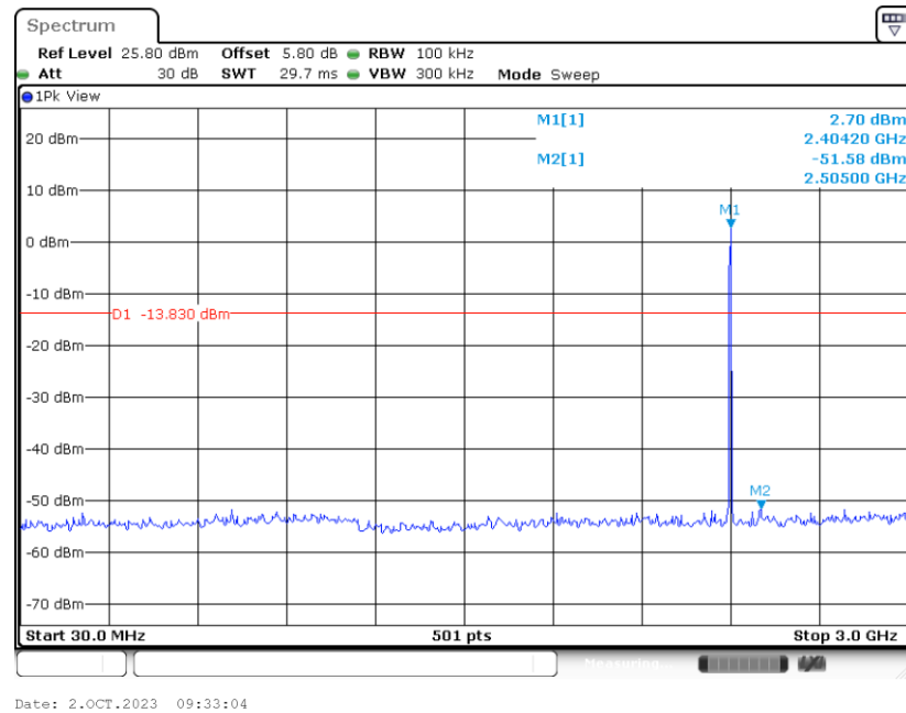
Conducted Spurious Emission Plot on GFSK Channel 00
