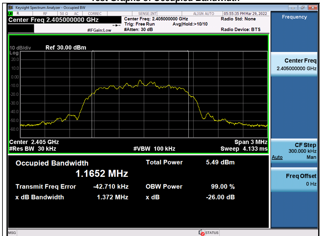
Test_Graph_LE1M_ANT1_2405_1Mbps_OBW
