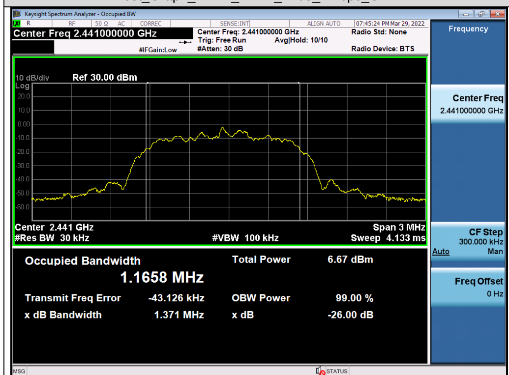
Test_Graph_LE1M_ANT1_2441_1Mbps_OBW
