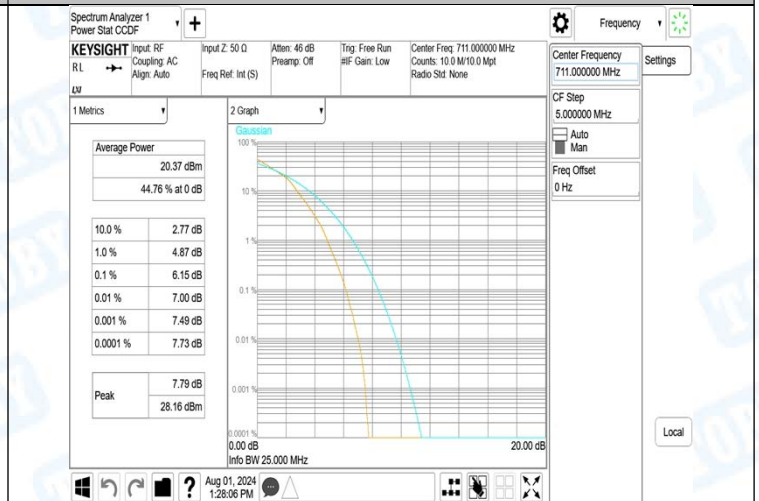
Band12-10MHz-16QAM-23130-27RB#0-PASS
