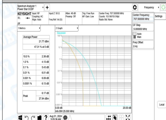
Band12-3MHz-QPSK-23165-1RB#0-PASS
