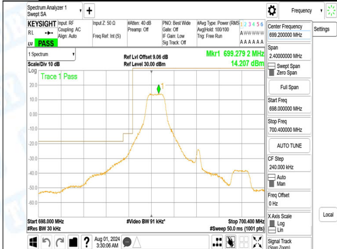
Band12_1.4MHz_16QAM_23017_6RB#0
