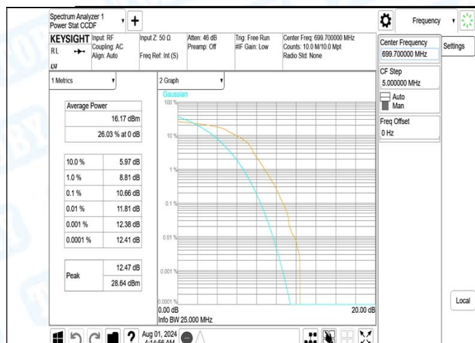
Band12-1.4MHz-16QAM-23095-1RB#0-PASS
