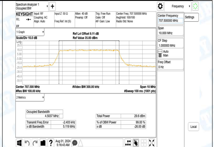
Band12-5MHz-16QAM-23035-25RB#0-PASS
