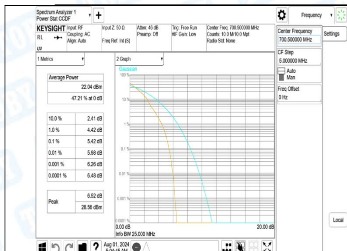
Band12-3MHz-QPSK-23095-1RB#0-PASS
