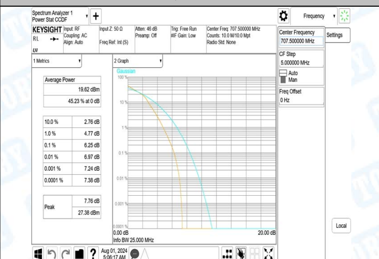
Band12-3MHz-16QAM-23165-15RB#0-PASS
