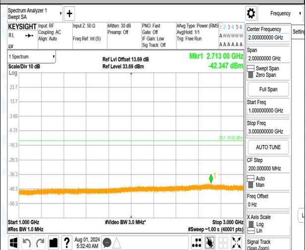
Band12_5MHz_16QAM_23095_1RB#0_1000~3000_1000~3000
