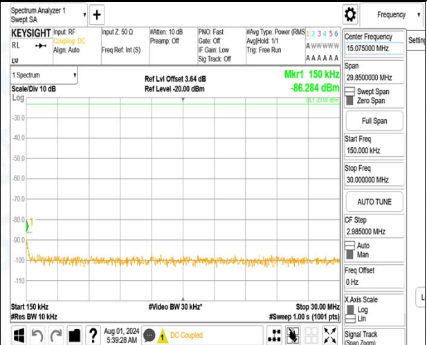
Band12_5MHz_QPSK_23155_1RB#0_1000~3000_1000~3000
