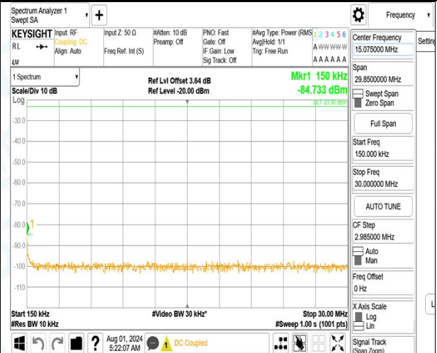
Band12_5MHz_QPSK_23035_1RB#0_1000~3000_1000~3000
